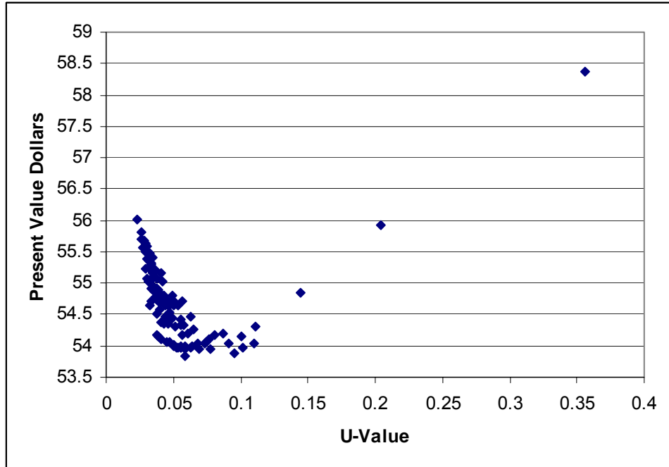
Figure 3 – Life-cycle Cost versus U-factor Curve of Wood-framed Walls in CZ 12
