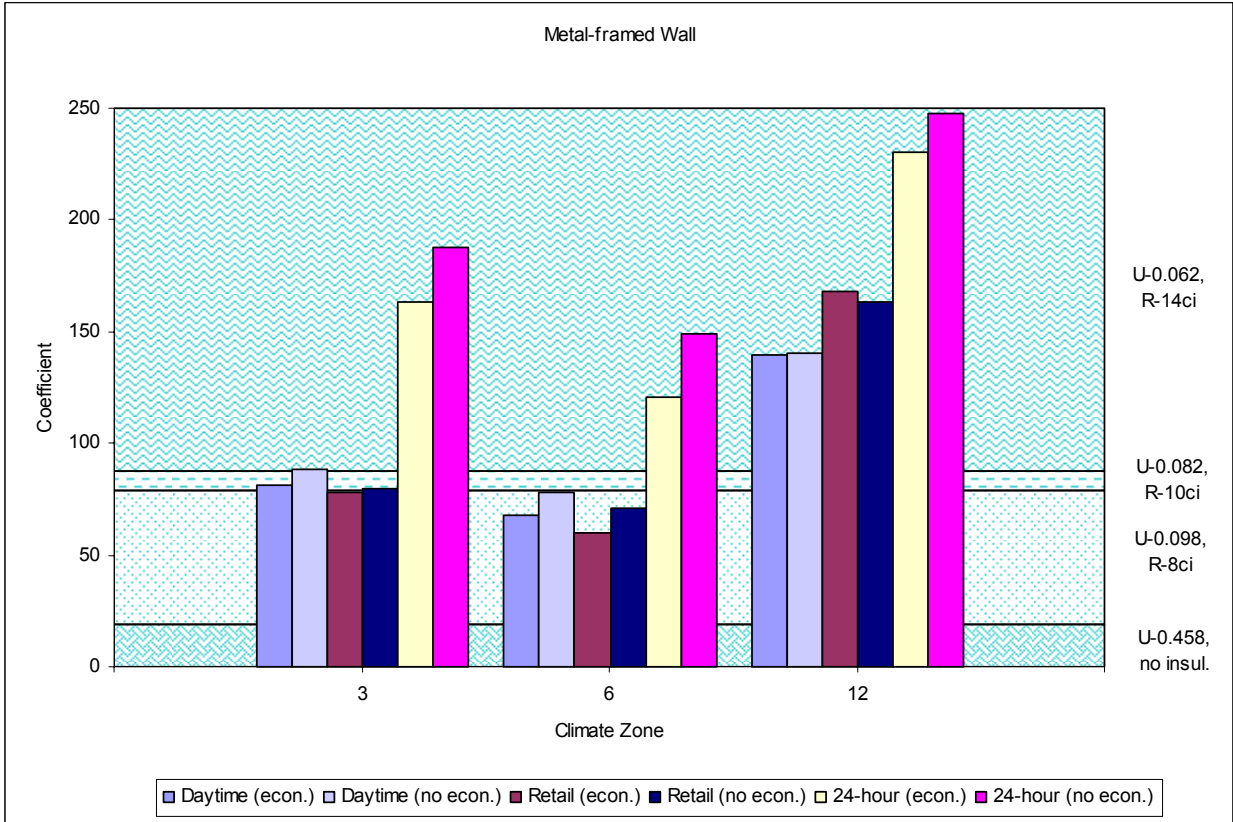
Figure 34 – Metal-framed Wall Coefficients (economizer sensitivity)
