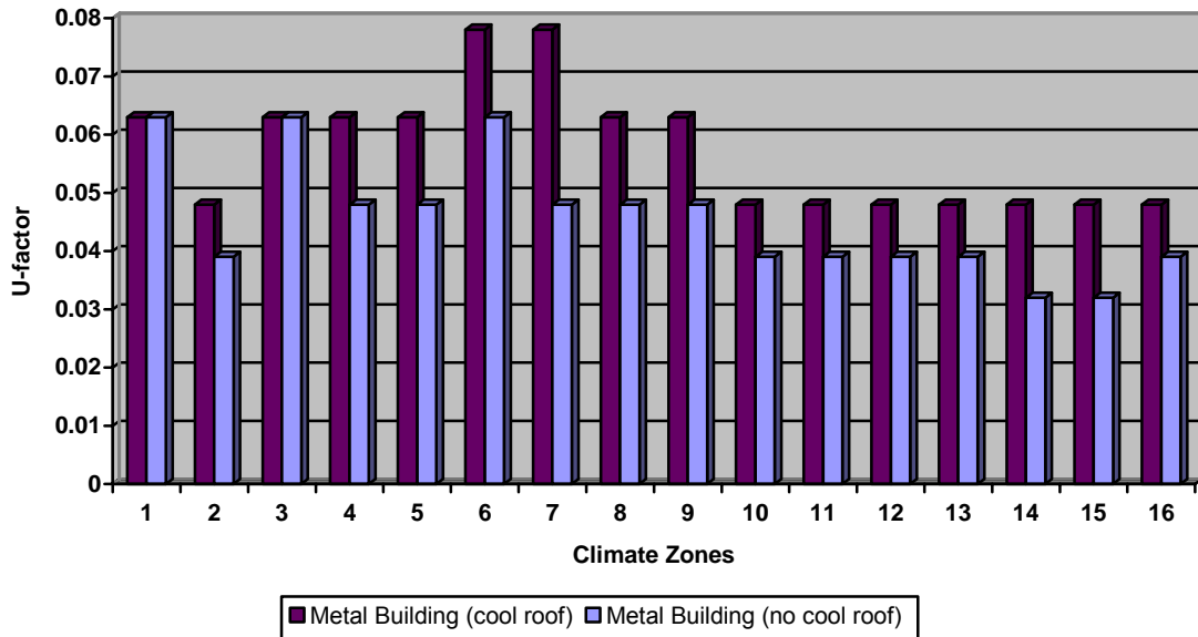
Figure 8 – Retail Roof Insulation Cool Roof Sensitivity Analysis for Metal Buildings
