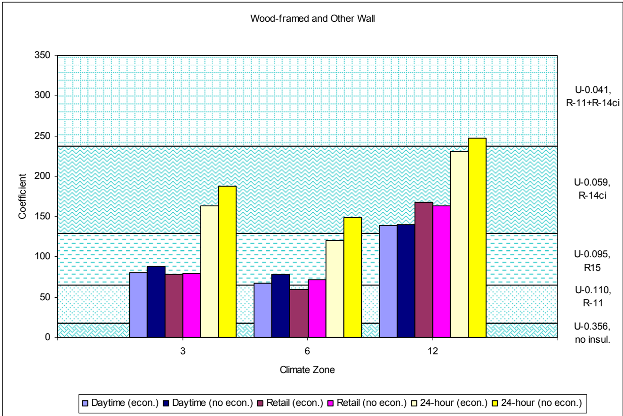
Figure 52 – Wood-framed and Other Wall Coefficients (economizer sensitivity)
