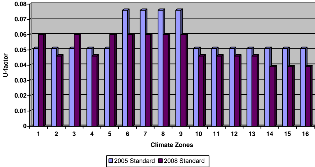
Figure 14 – Wood-framed and Other Roof (Daytime) Statewide Energy Impacts ( \text{ft}^2\text{-yr} ): TDV=0.838, kWh=0.027, therm=0.002
