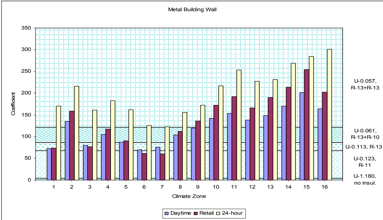
Figure 28 – Metal Building Wall Coefficients
