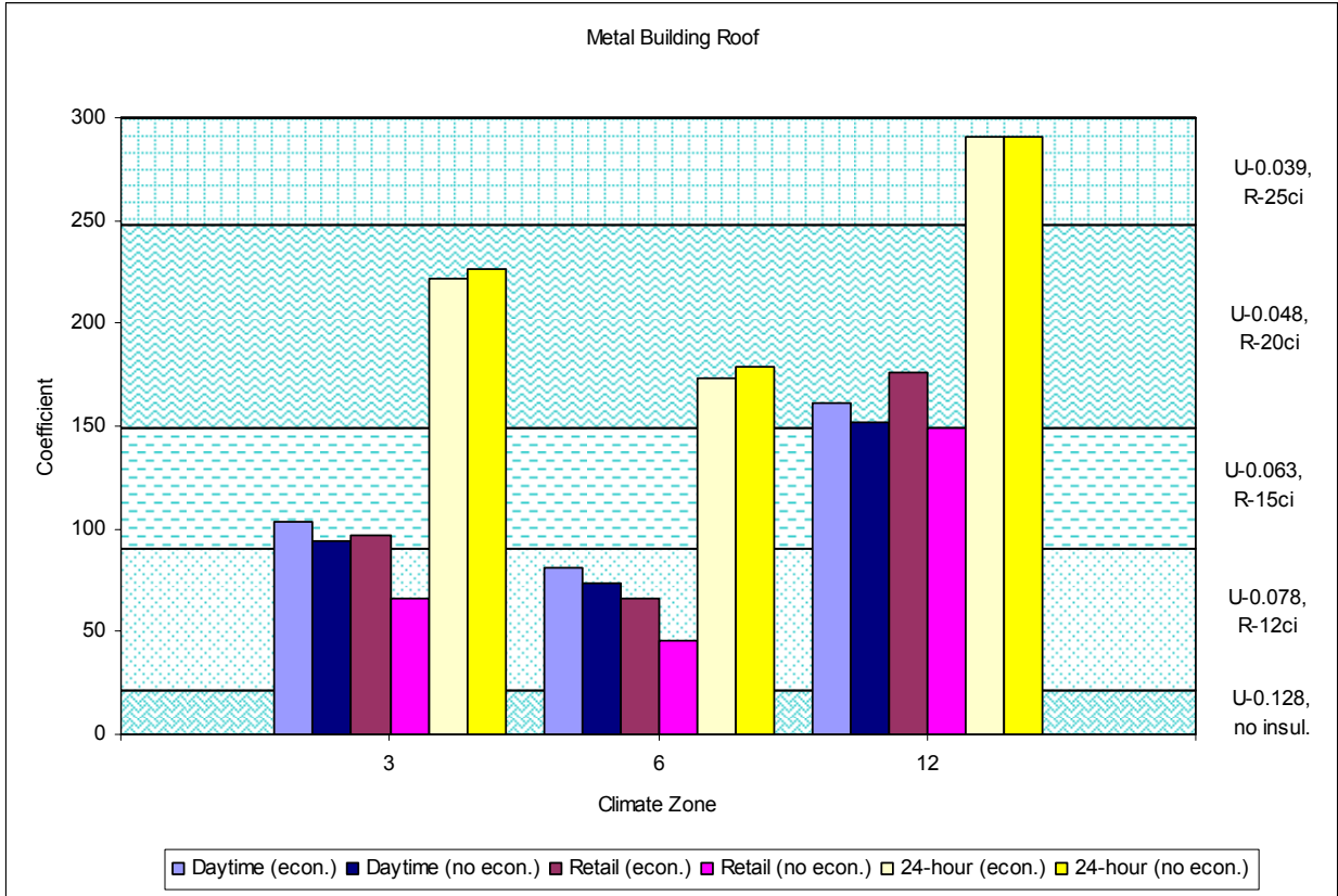
Figure 13 – Metal Building Roof Coefficients (economizer sensitivity)
