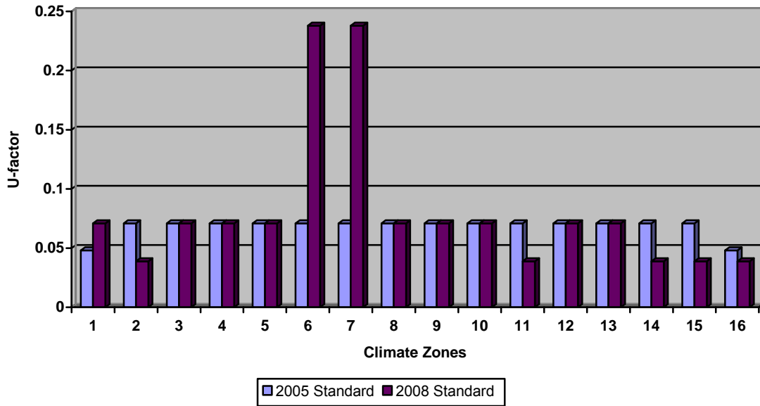
Figure 59 – Other Floor (Daytime) Statewide Energy Impacts (ft 2 -yr): TDV=0.218, kWh=0.036, therm=-0.003
