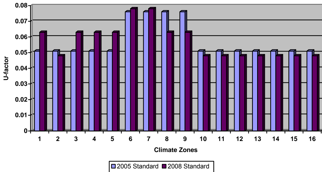
Figure 5 –Metal Building Roof (Retail) Statewide Energy Impacts (ft 2 -yr): TDV=0.305, kWh=0.015, therm=0.000
