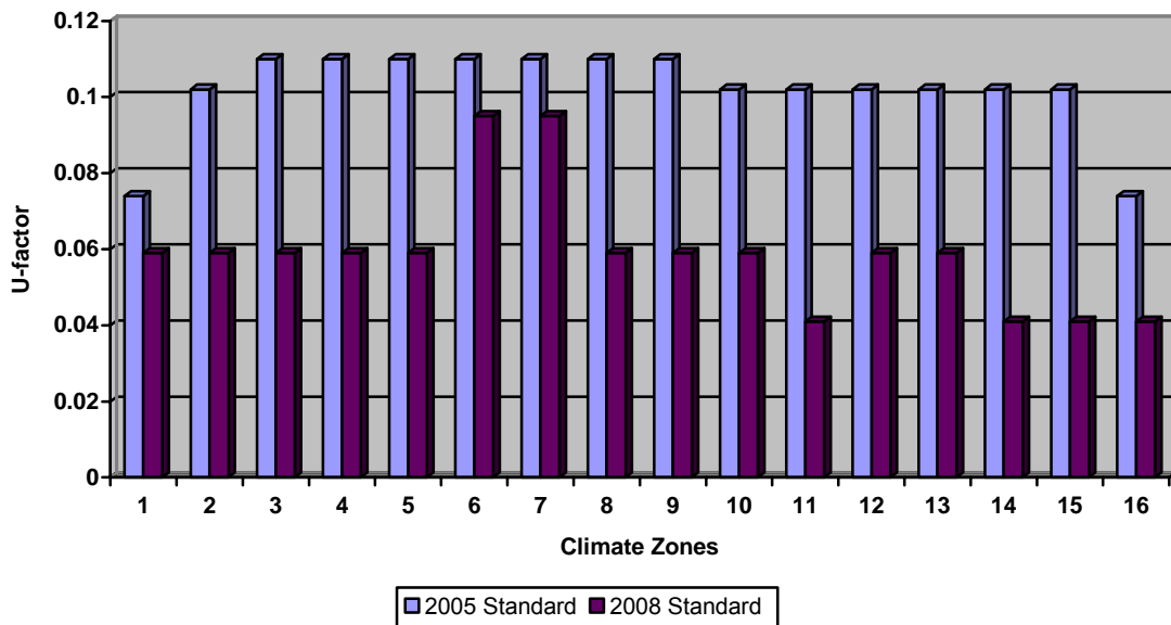
Figure 49 – Wood-framed and Other Wall (24-hour) Statewide Energy Impacts ( ft^2\text{-yr} ): TDV=7.644, kWh=0.394, therm=0.027
