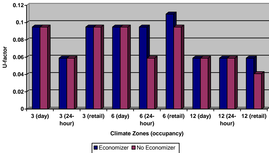
Figure 50 – Daytime Economizer Insulation Sensitivity Analysis for Wood-framed and Other Wall
