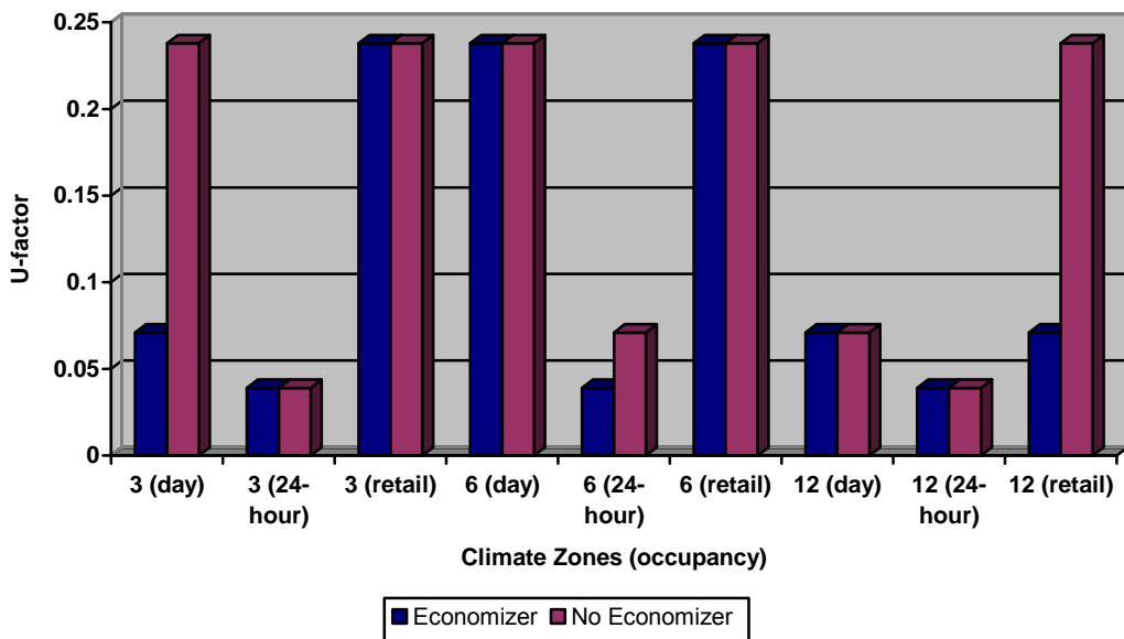
Figure 62 – Daytime Economizer Insulation Sensitivity Analysis for Other Floor
