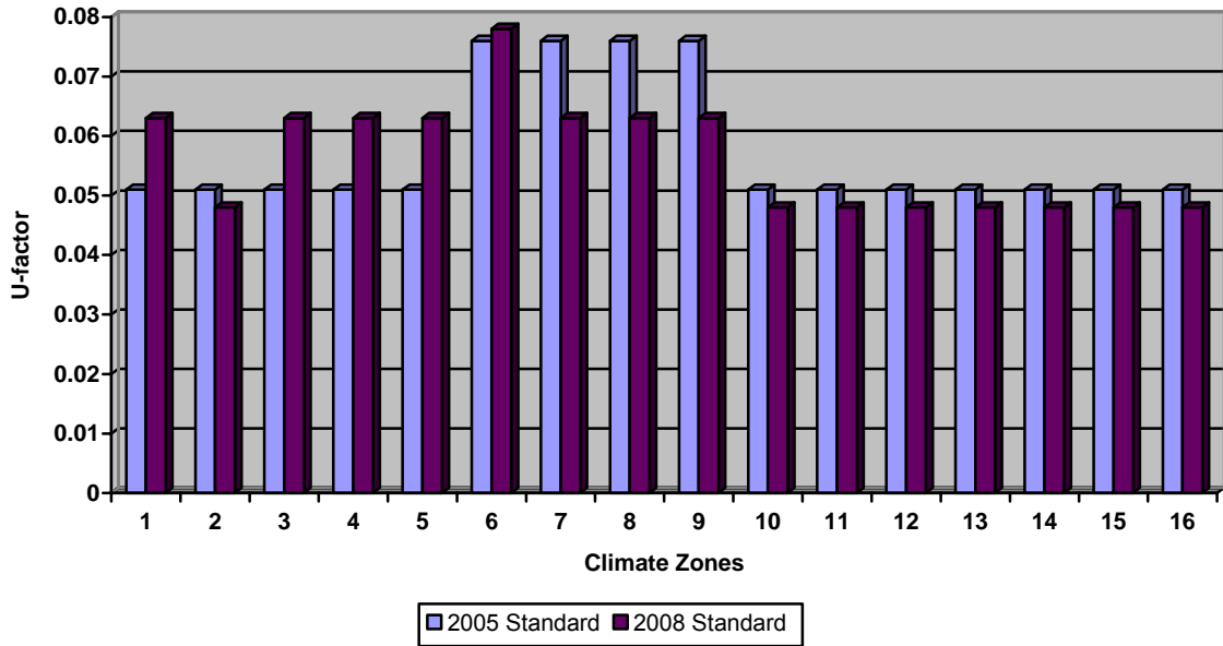
Figure 4 –Metal Building Roof (Daytime) Statewide Energy Impacts (ft 2 -yr): TDV=0.222, kWh=0.010, therm=0.000
