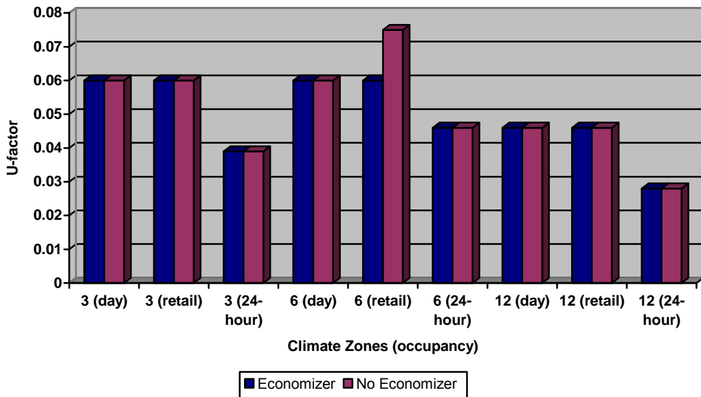
Figure 20 – Economizer Insulation Sensitivity Analysis for Wood-framed and Other Roof
