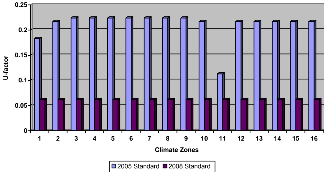
Figure 32 – Metal-framed Wall (24-hour) Statewide Energy Impacts (ft 2 -yr): TDV=28.985, kWh=1.524, therm=0.103
