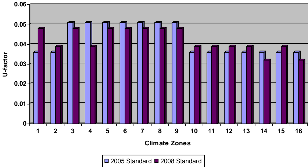
Figure 6 – Metal Building Roof (24-hour) Statewide Energy Impacts (ft 2 -yr): TDV=3.761, kWh=0.112, therm=0.016
