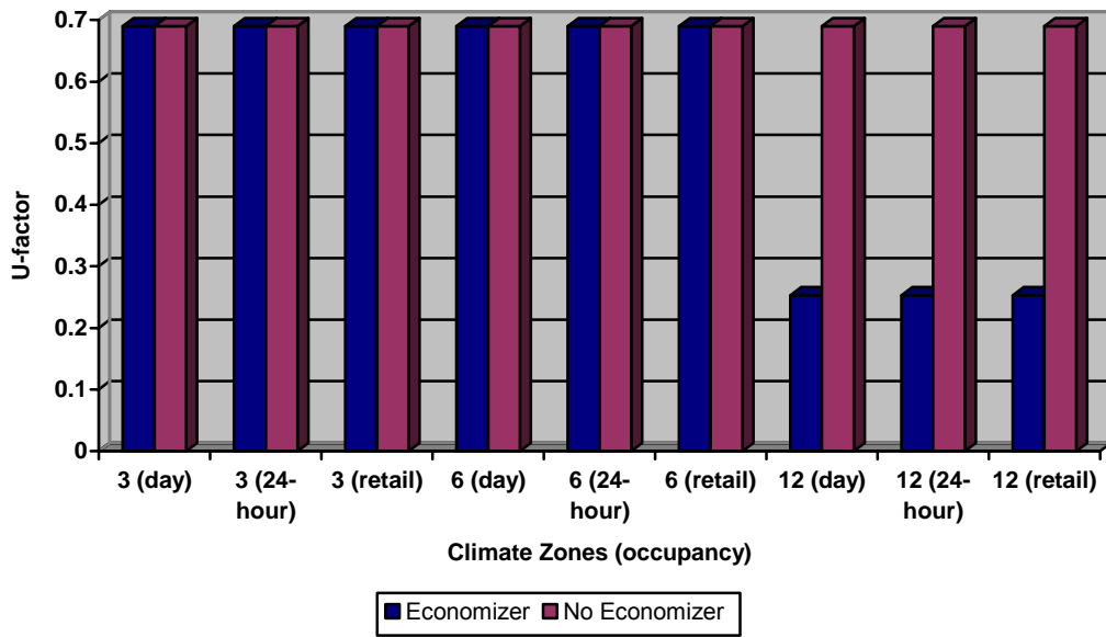
Figure 44 – Daytime Economizer Insulation Sensitivity Analysis for Mass (15.0≤HC) Wall
