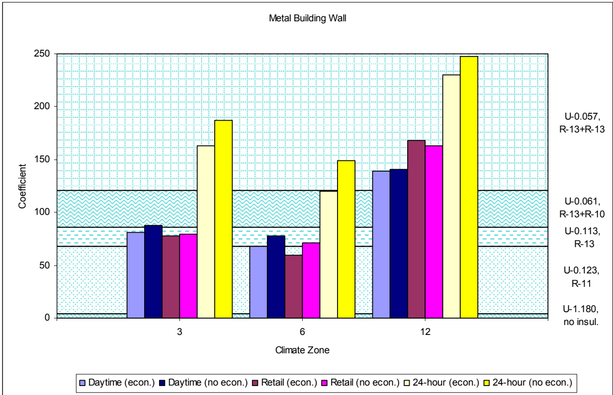
Figure 29 – Metal Building Wall Coefficients (economizer sensitivity)
