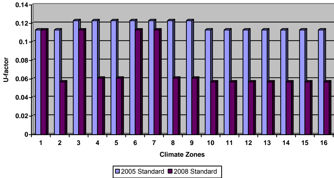
Figure 24 – Metal Building Wall (Daytime) Statewide Energy Impacts ( ft^2 -yr): TDV=5.554, kWh=0.262, therm=0.013
