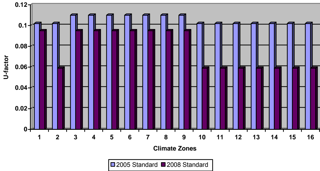
Figure 47 – Wood-framed and Other Wall (Daytime) Statewide Energy Impacts ( \text{ft}^2\text{-yr} ): TDV=3.428, kWh=0.159, therm=0.006
