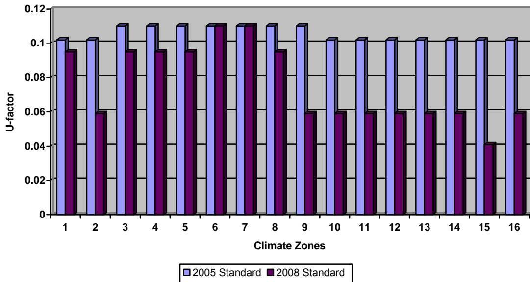
Figure 48 – Wood-framed and Other Wall (Retail) Statewide Energy Impacts ( \text{ft}^2\text{-yr} ): TDV=4.825, kWh=0.263, therm=0.010
