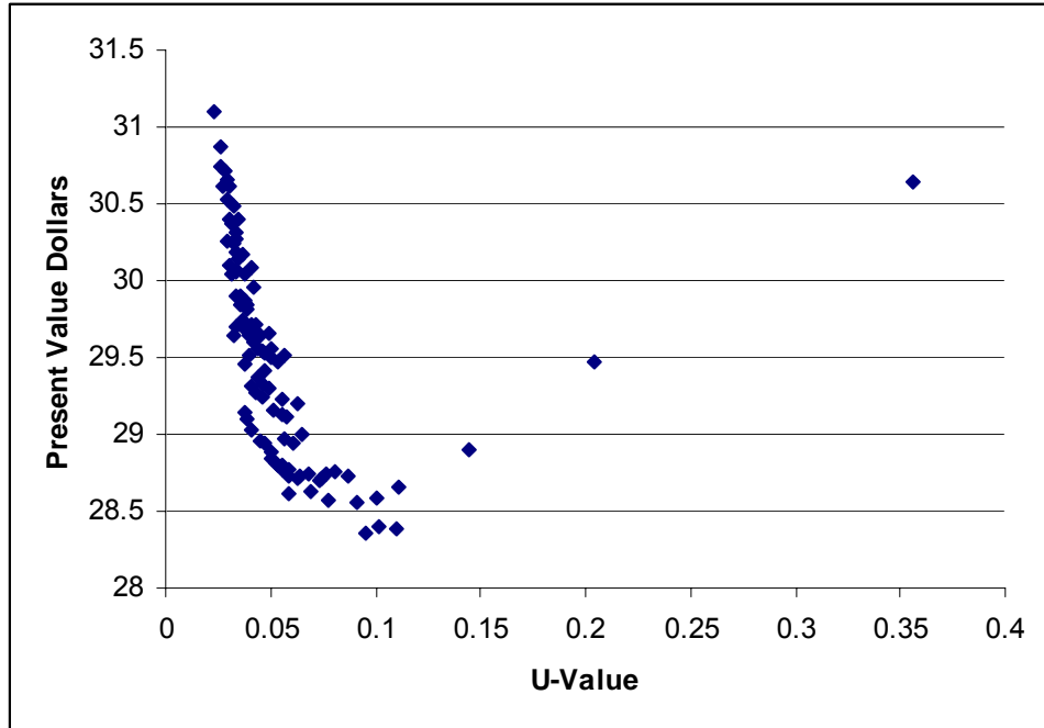
Figure 2 – Life-cycle Cost versus U-factor Curve of Wood-framed Walls in CZ 3
