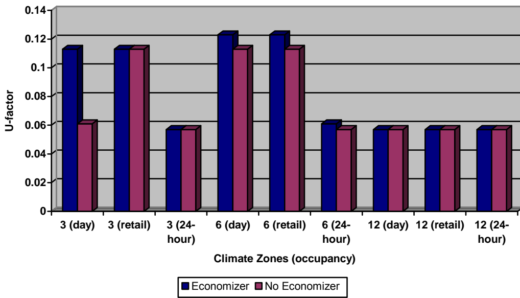
Figure 27 – Economizer Insulation Sensitivity Analysis for Metal Building Wall
