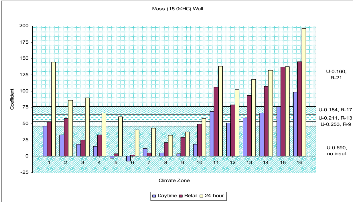
Figure 45 – Mass (15.0≤HC) Wall Coefficients
