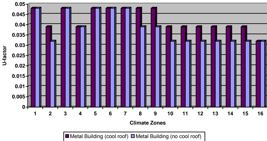
Figure 9 – 24-hour Roof Insulation Cool Roof Sensitivity Analysis for Metal Buildings
