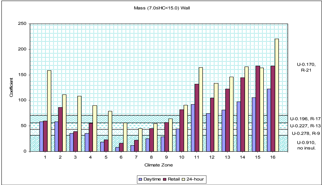
Figure 39 – Mass (7.0≤HC<15.0) Wall Coefficients
