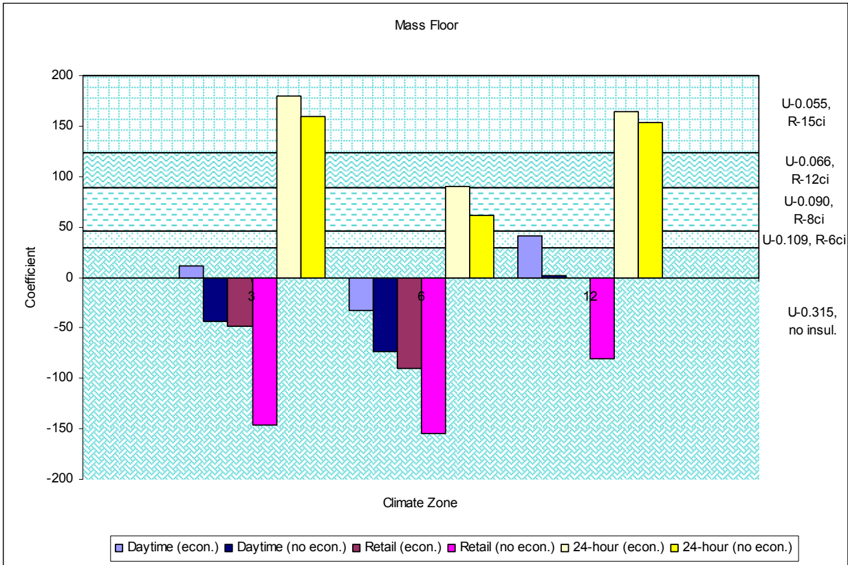
Figure 58 – Mass Floor Coefficients (economizer sensitivity)
