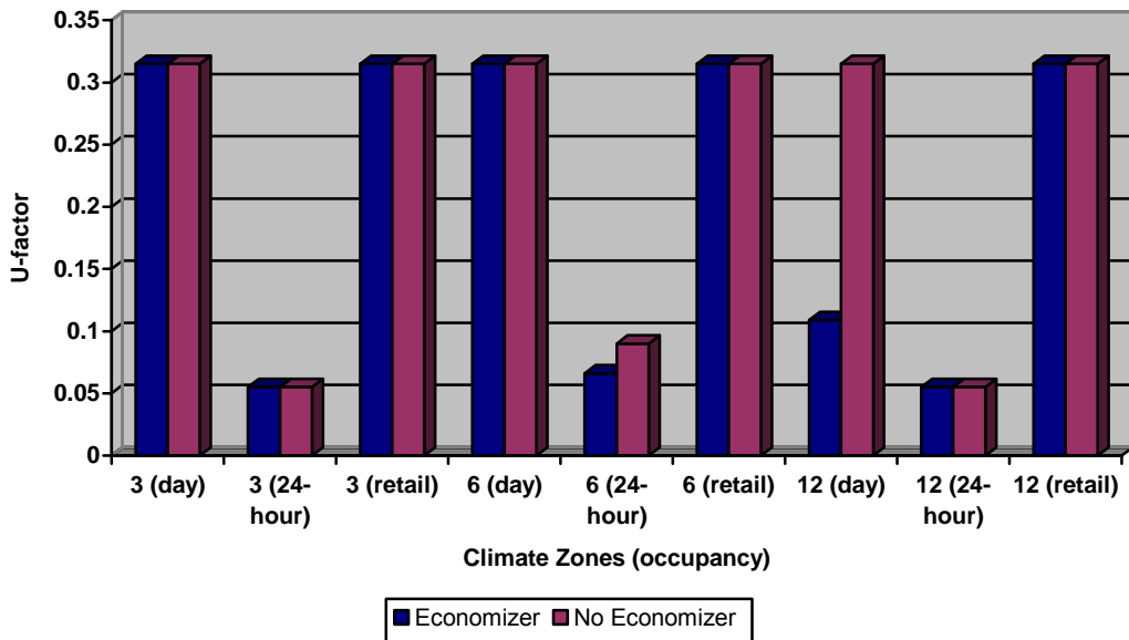
Figure 56 – Daytime Economizer Insulation Sensitivity Analysis for Mass Floor
