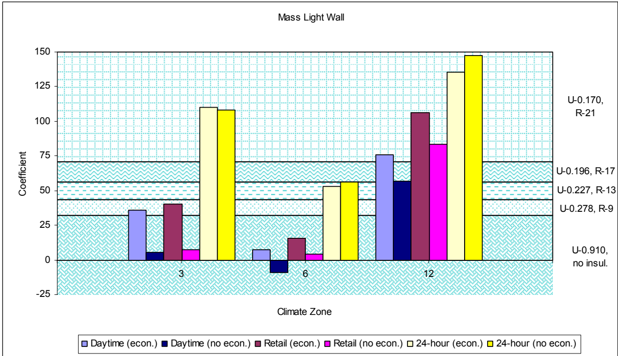
Figure 40 – Mass (7.0≤HC<15.0) Wall Coefficients (economizer sensitivity)
