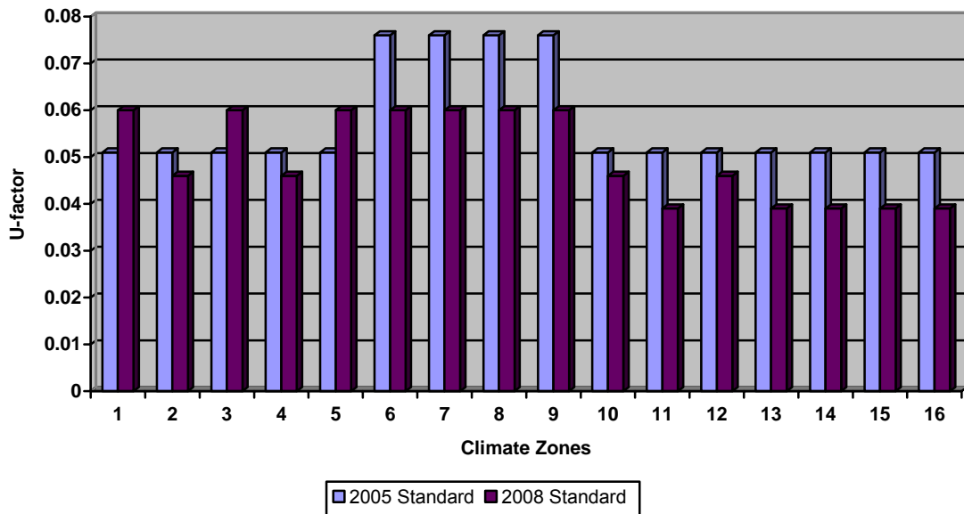
Figure 15 – Wood-framed and Other Roof (Retail) Statewide Energy Impacts ( \text{ft}^2\text{-yr} ): TDV=1.088, kWh=0.042, therm=0.003
