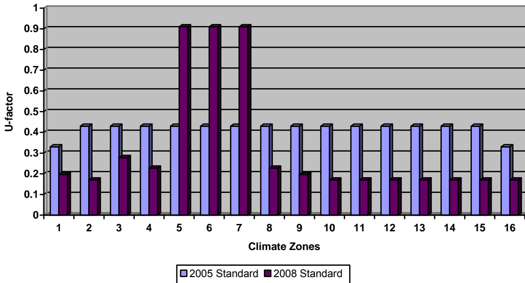
Figure 36 – Mass (7.0≤HC<15.0) Wall (Retail) Statewide Energy Impacts (ft 2 -yr): TDV=12.603, kWh=0.507, therm=0.040
