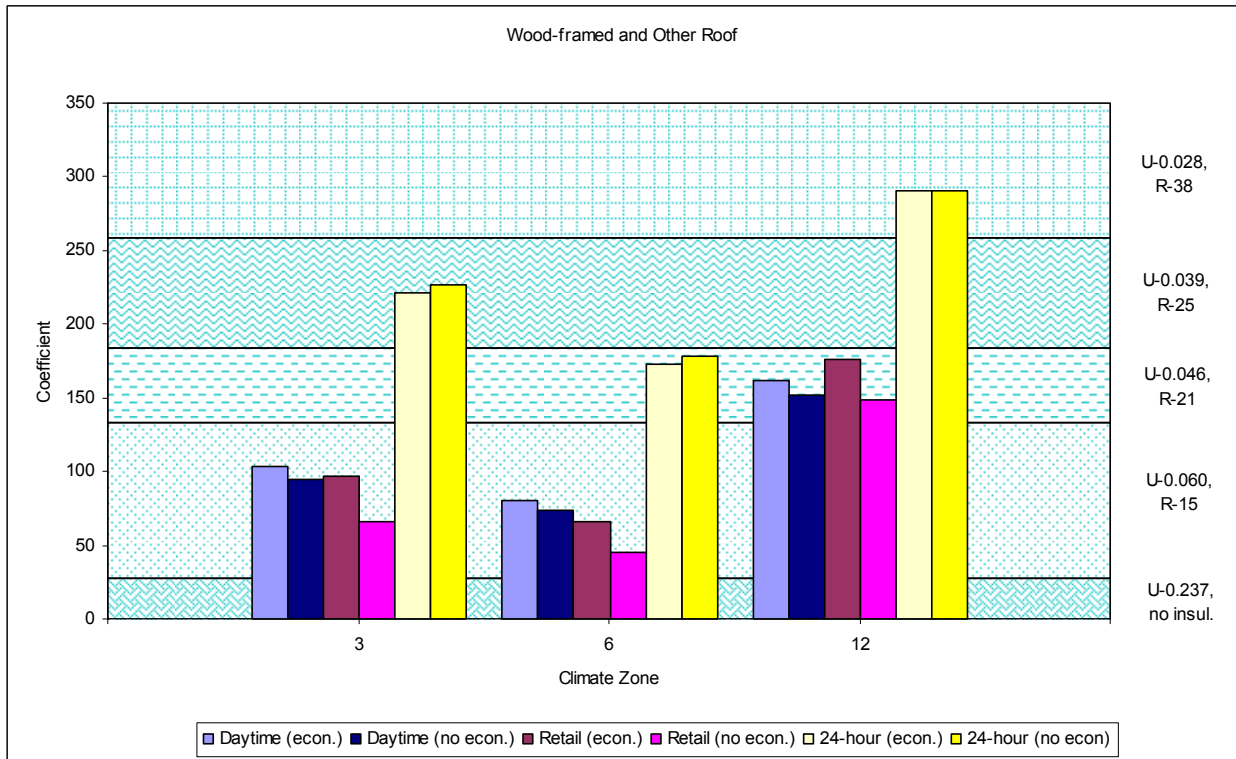
Figure 23 – Wood-framed and Other Roof Coefficients (economizer sensitivity)
