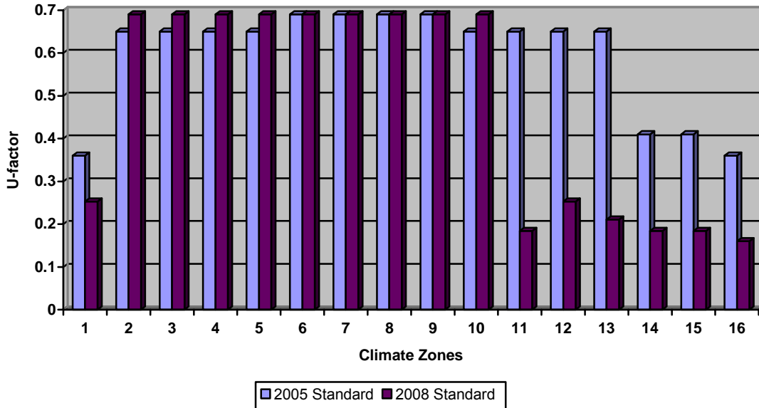
Figure 43 – Mass (15.0≤HC) Wall (24-hour) Statewide Energy Impacts (ft 2 -yr): TDV=8.626, kWh=0.198, therm=0.038
