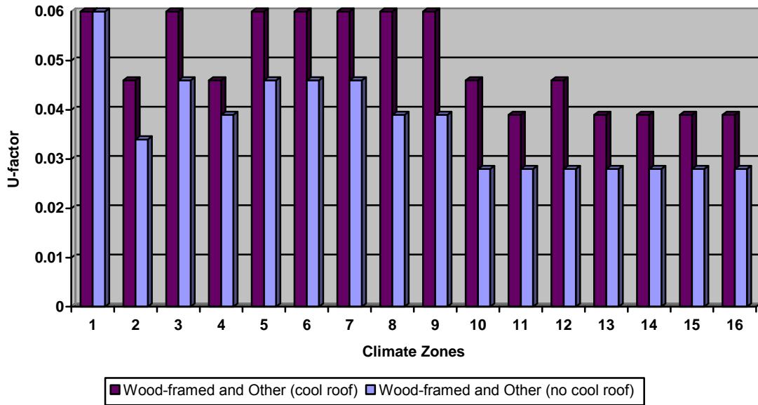
Figure 18 – Retail Roof Insulation Cool Roof Sensitivity Analysis for Wood-framed and Other
