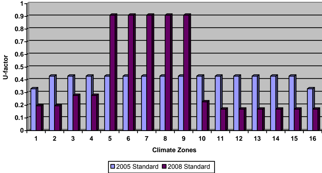
Figure 35 – Mass (7.0≤HC<15.0) Wall (Daytime) Statewide Energy Impacts (ft 2 -yr): TDV=4.311, kWh=0.066, therm=0.016
