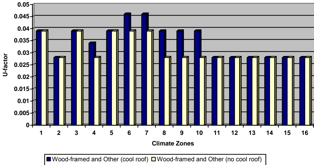
Figure 19 – 24-hour Roof Insulation Cool Roof Sensitivity Analysis for Wood-framed and Other
