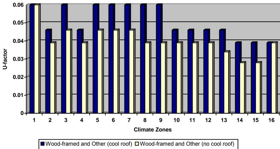
Figure 17 – Daytime Roof Insulation Cool Roof Sensitivity Analysis for Wood-framed and Other
