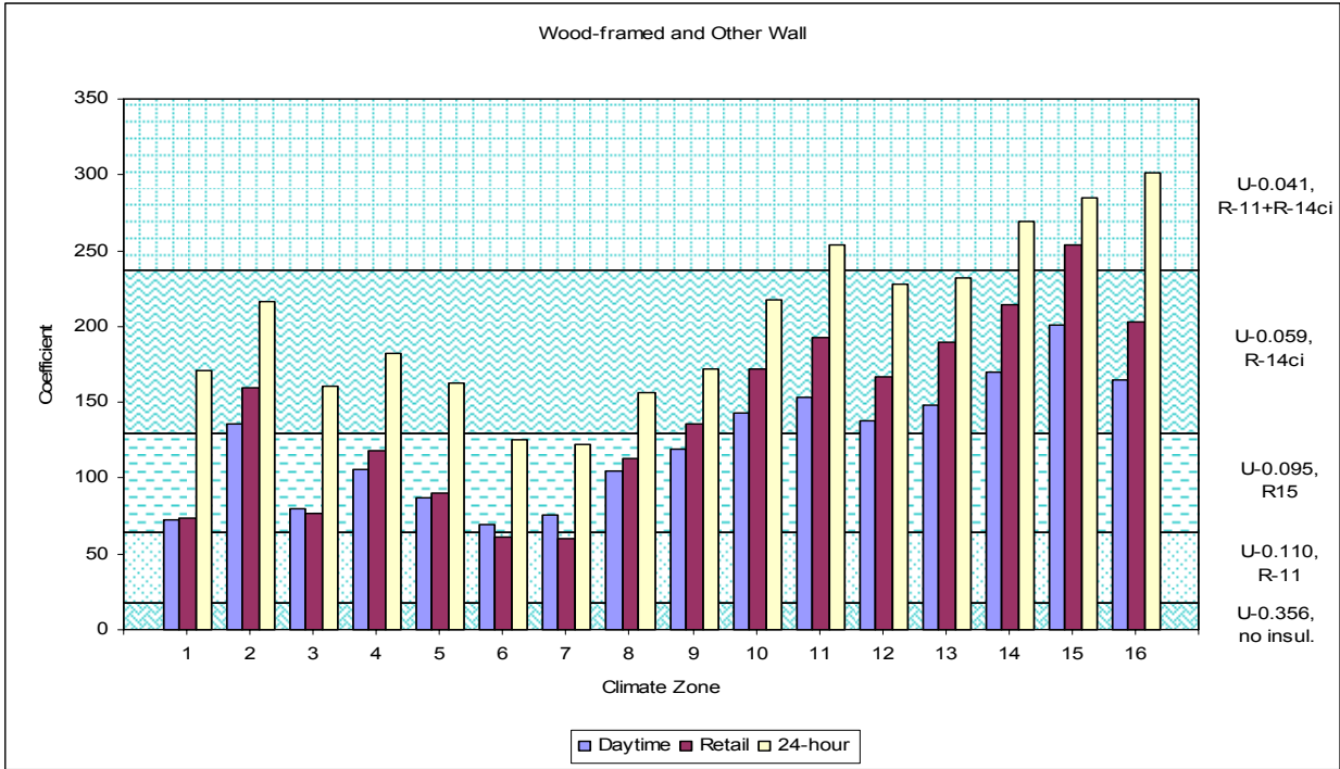
Figure 51 – Wood-framed and Other Wall Coefficients
