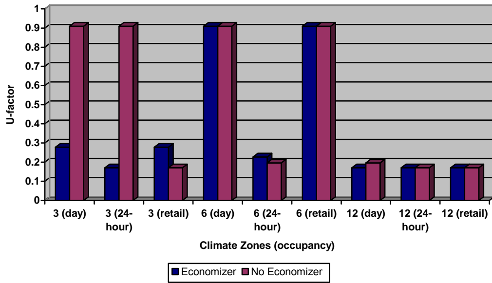
Figure 38 – Economizer Insulation Sensitivity Analysis for Mass ( 7.0 \leq HC < 15.0 ) Wall
