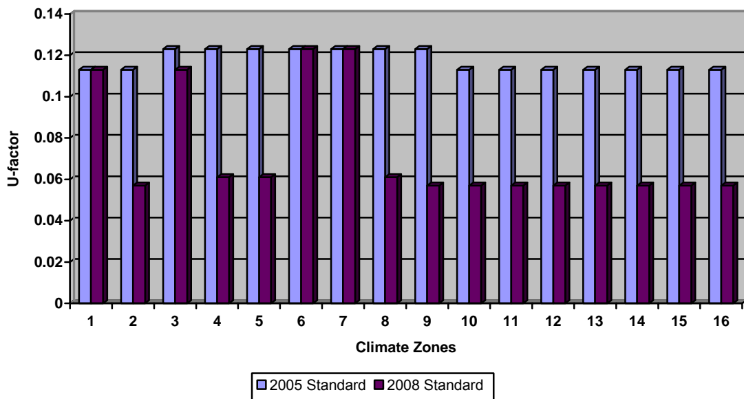
Figure 25 – Metal Building Wall (Retail) Statewide Energy Impacts ( ft^2 -yr): TDV=6.800, kWh=0.373, therm=0.014
