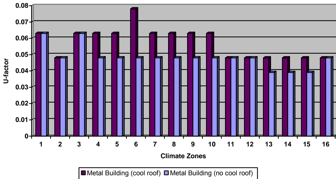
Figure 7 – Daytime Roof Insulation Cool Roof Sensitivity Analysis for Metal Buildings
