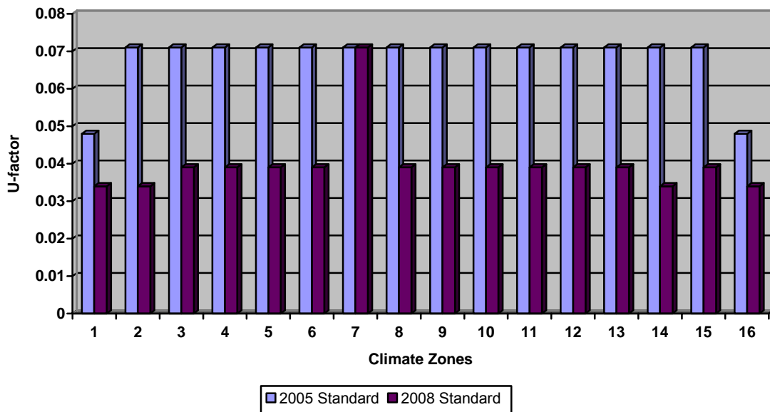
Figure 61 – Other Floor (24-hour) Statewide Energy Impacts (ft 2 -yr): TDV=5.188, kWh=0.058, therm=0.029
