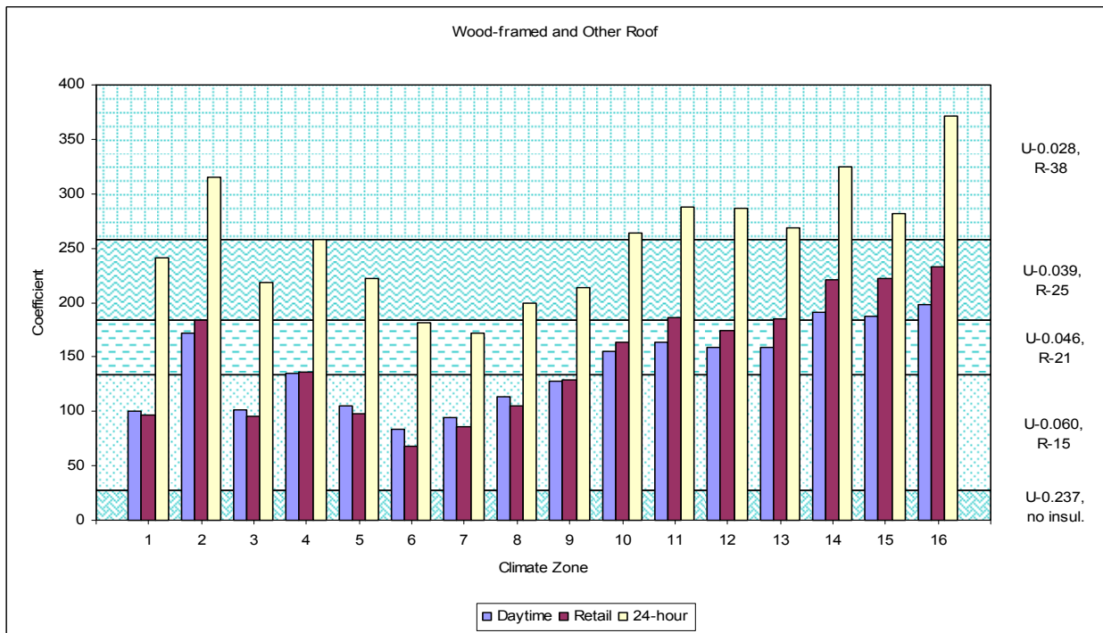
Figure 21 – Wood-framed and Other Roof Coefficients
