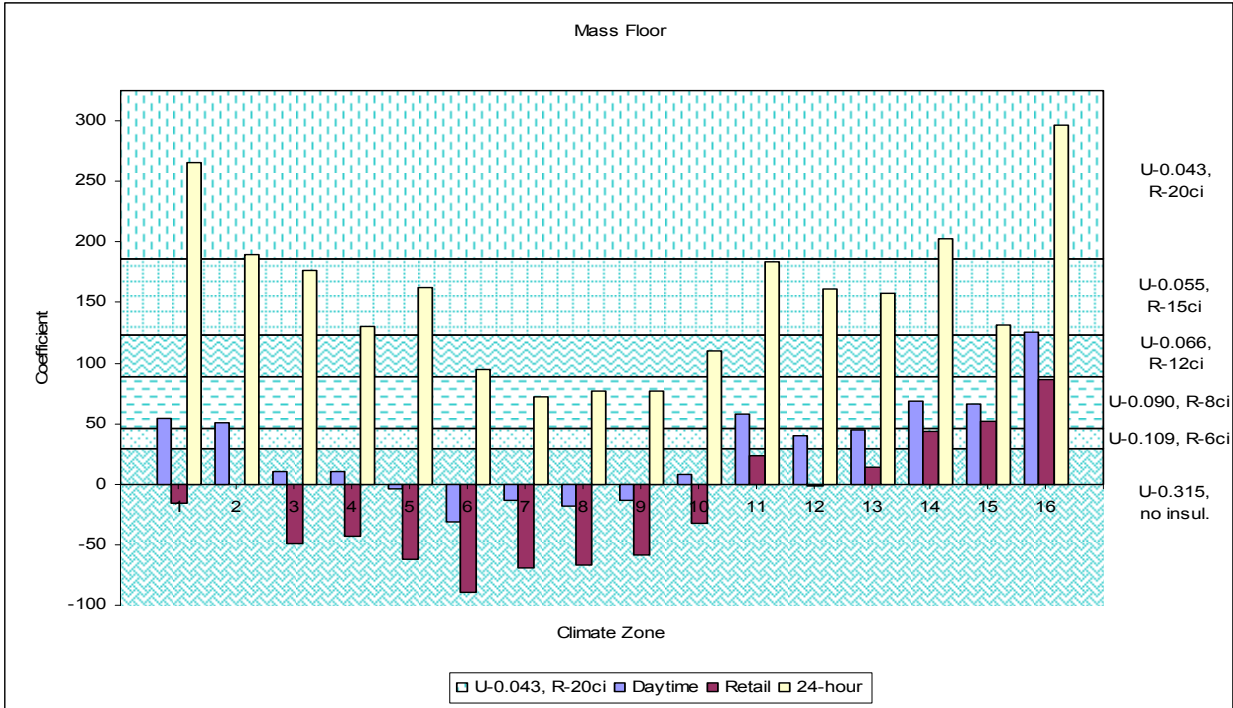
Figure 57 – Mass Floor Coefficients
