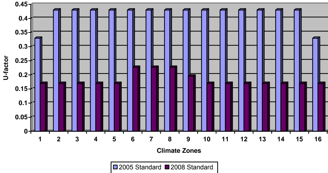
Figure 37 – Mass ( 7.0 \leq HC < 15.0 ) Wall (24-hour) Statewide Energy Impacts ( ft^2 -yr): TDV=23.344, kWh=0.500, therm=0.118
