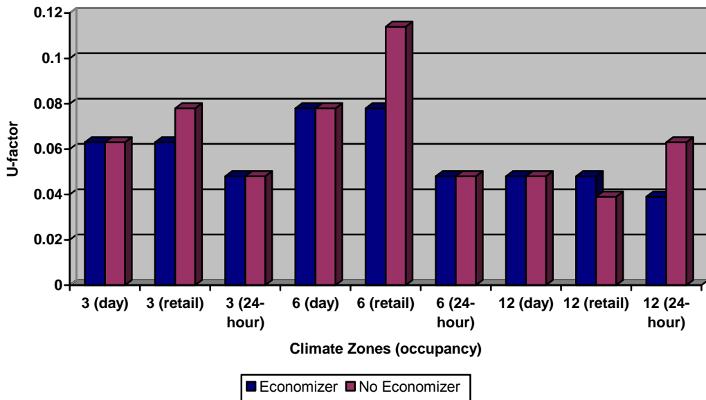
Figure 10 – Economizer Insulation Sensitivity Analysis for Metal Building Roof
