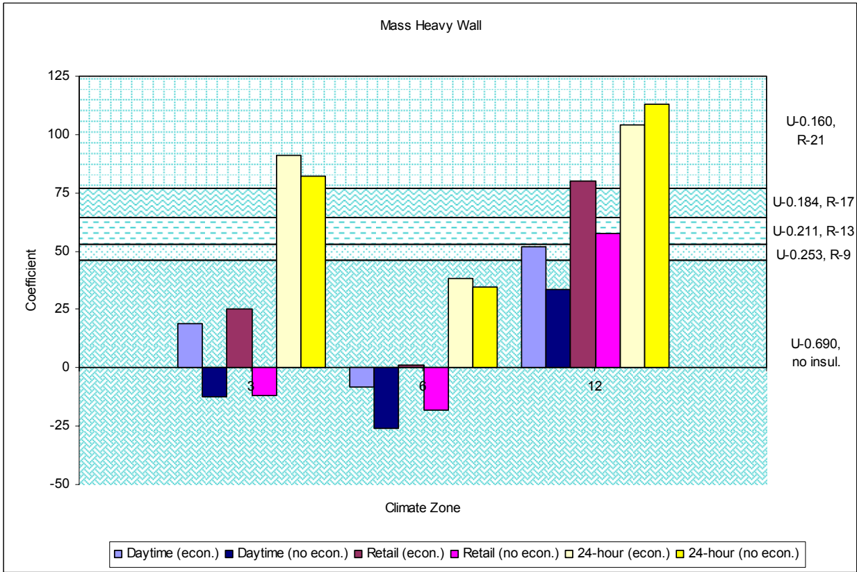
Figure 46 – Mass (15.0≤HC) Wall Coefficients (economizer sensitivity)
