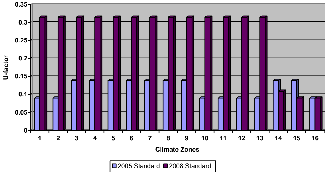
Figure 54 – Mass Floor (Retail) Statewide Energy Impacts (ft 2 -yr): TDV=6.200, kWh=0.472, therm=-0.026
