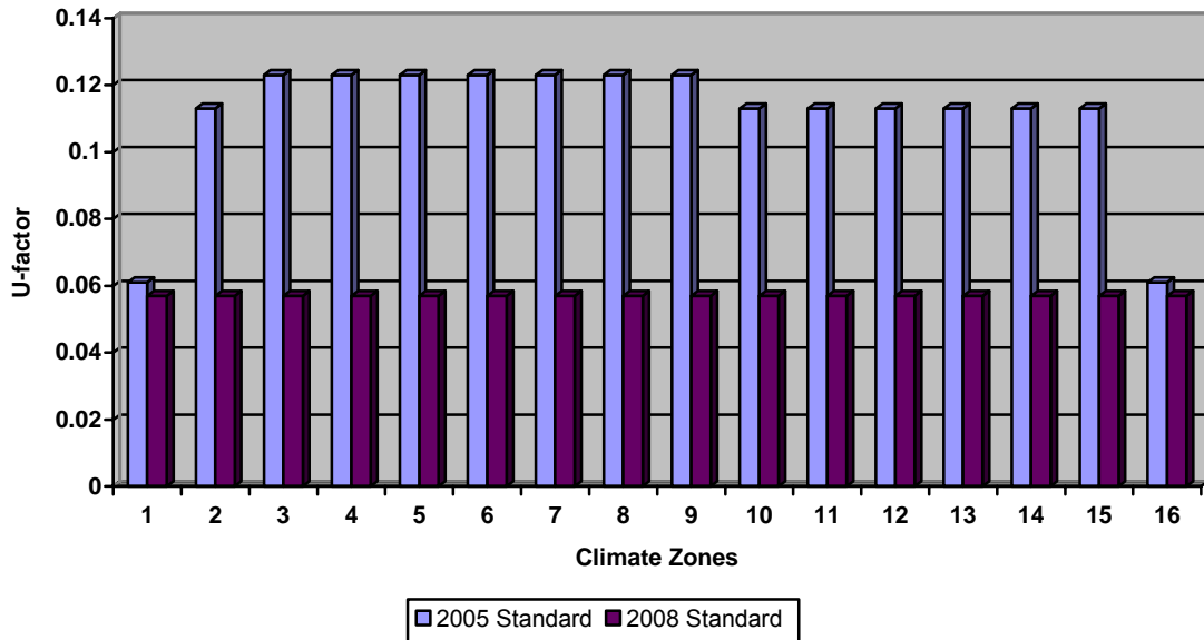
Figure 26 – Metal Building Wall (24-hour) Statewide Energy Impacts (ft 2 -yr): TDV=11.138, kWh=0.586, therm=0.040
