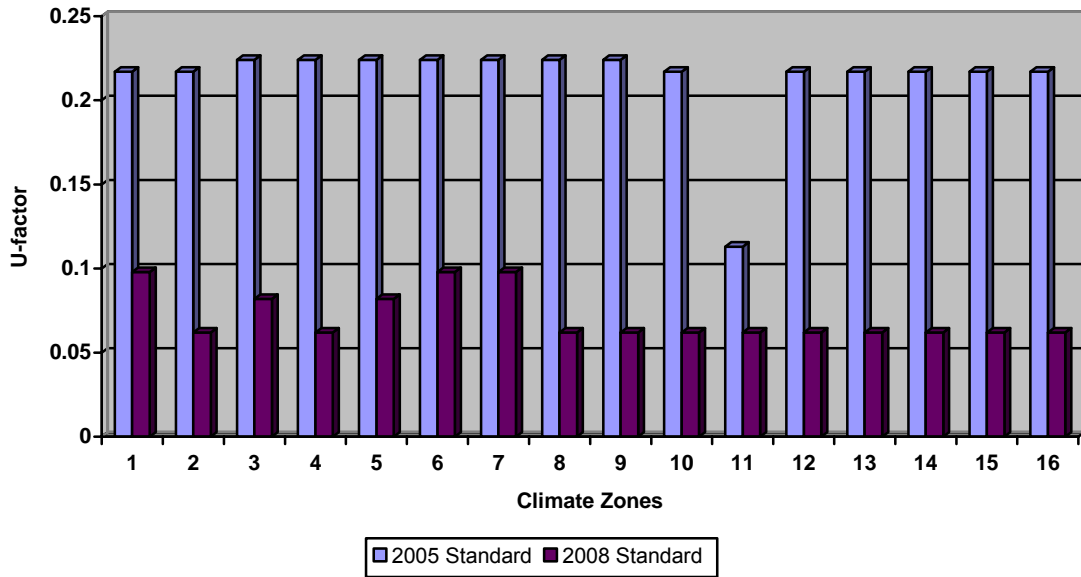
Figure 30 – Metal-framed Wall (Daytime) Statewide Energy Impacts (ft 2 -yr): TDV=17.505, kWh=0.821, therm=0.044
