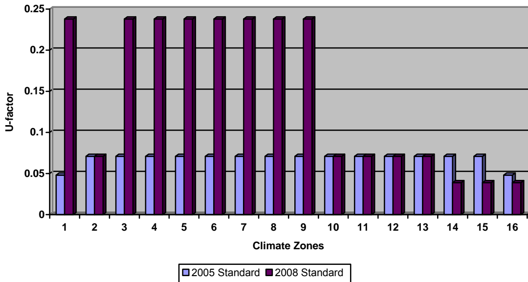
Figure 60 – Other Floor (Retail) Statewide Energy Impacts (ft 2 -yr): TDV=2.218, kWh=0.151, therm=-0.012
