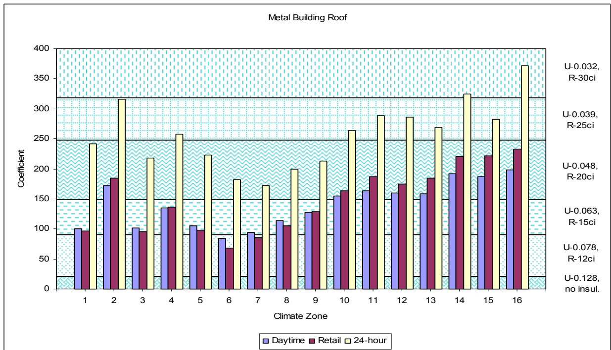
Figure 11 – Metal Building Roof Coefficients (cool roofs)
