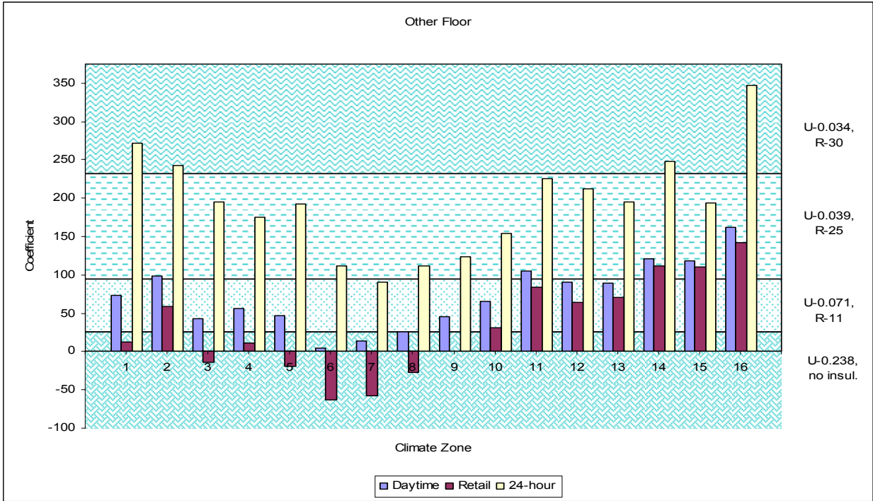
Figure 63 – Other Floor Coefficients
