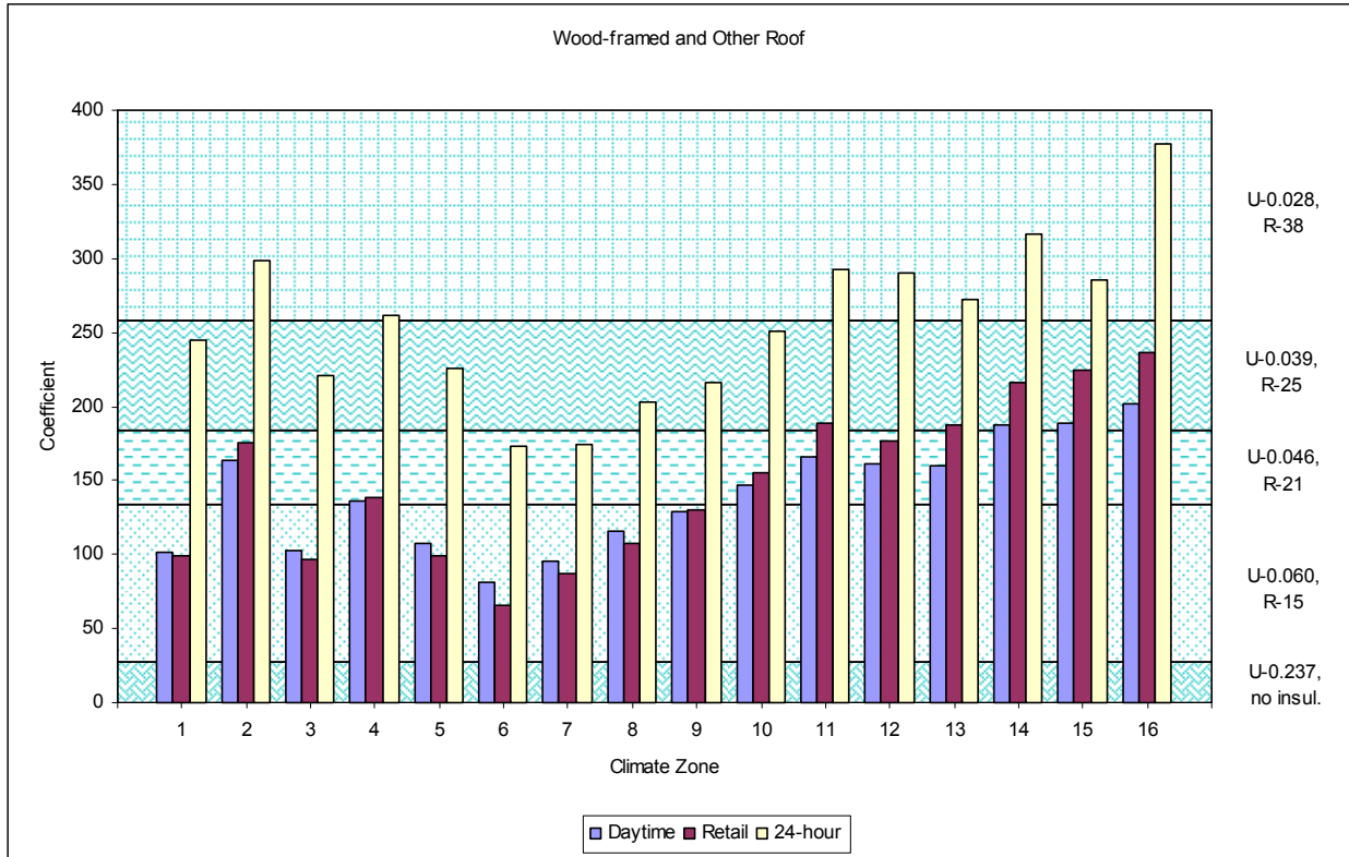
Figure 22 – Wood-framed and Other Roof Coefficients (no cool roof)
