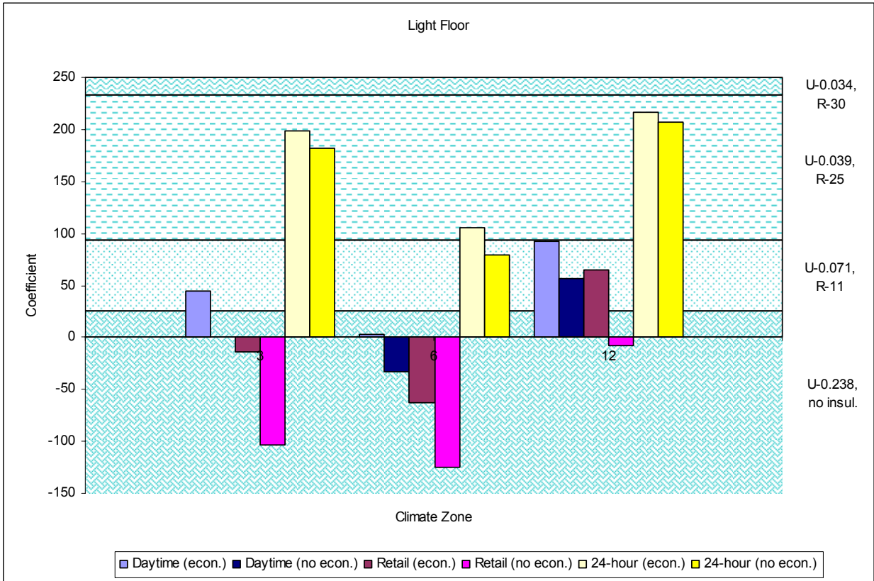
Figure 64 – Other Floor Coefficients (economizer sensitivity)
