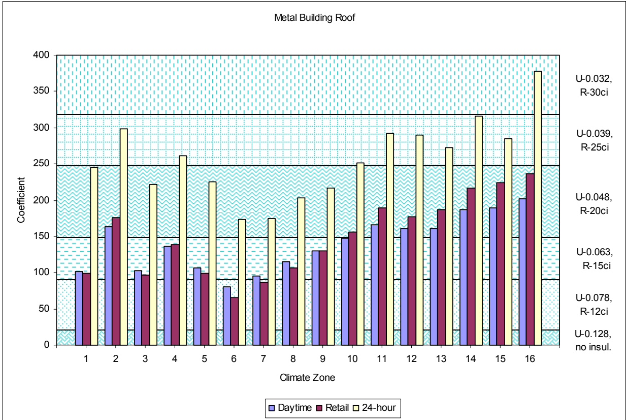
Figure 12 – Metal Building Roof Coefficients (no cool roof)
