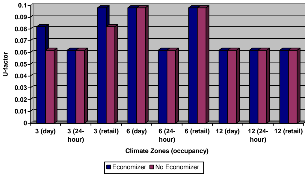
Figure 33 – Economizer Insulation Sensitivity Analysis for Metal-framed Wall
