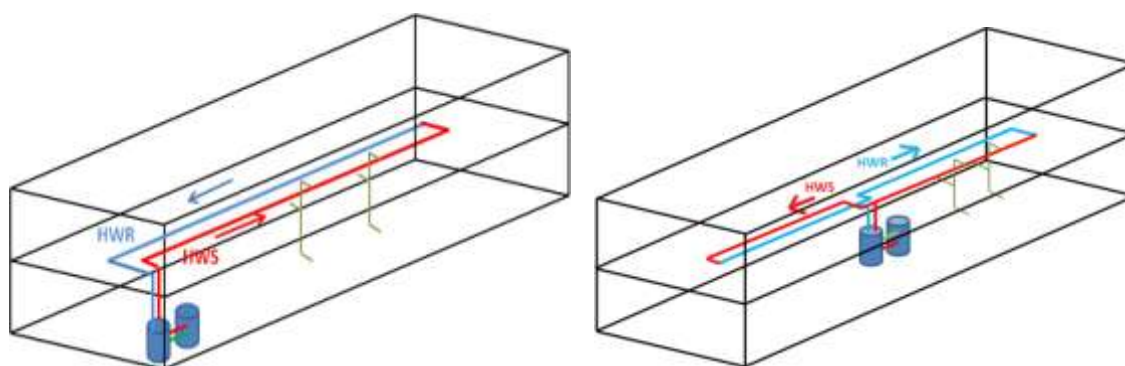
Figure 8. Low-rise Prototype Recirculation Piping Default (Left) and Optimized (Right) Configurations
