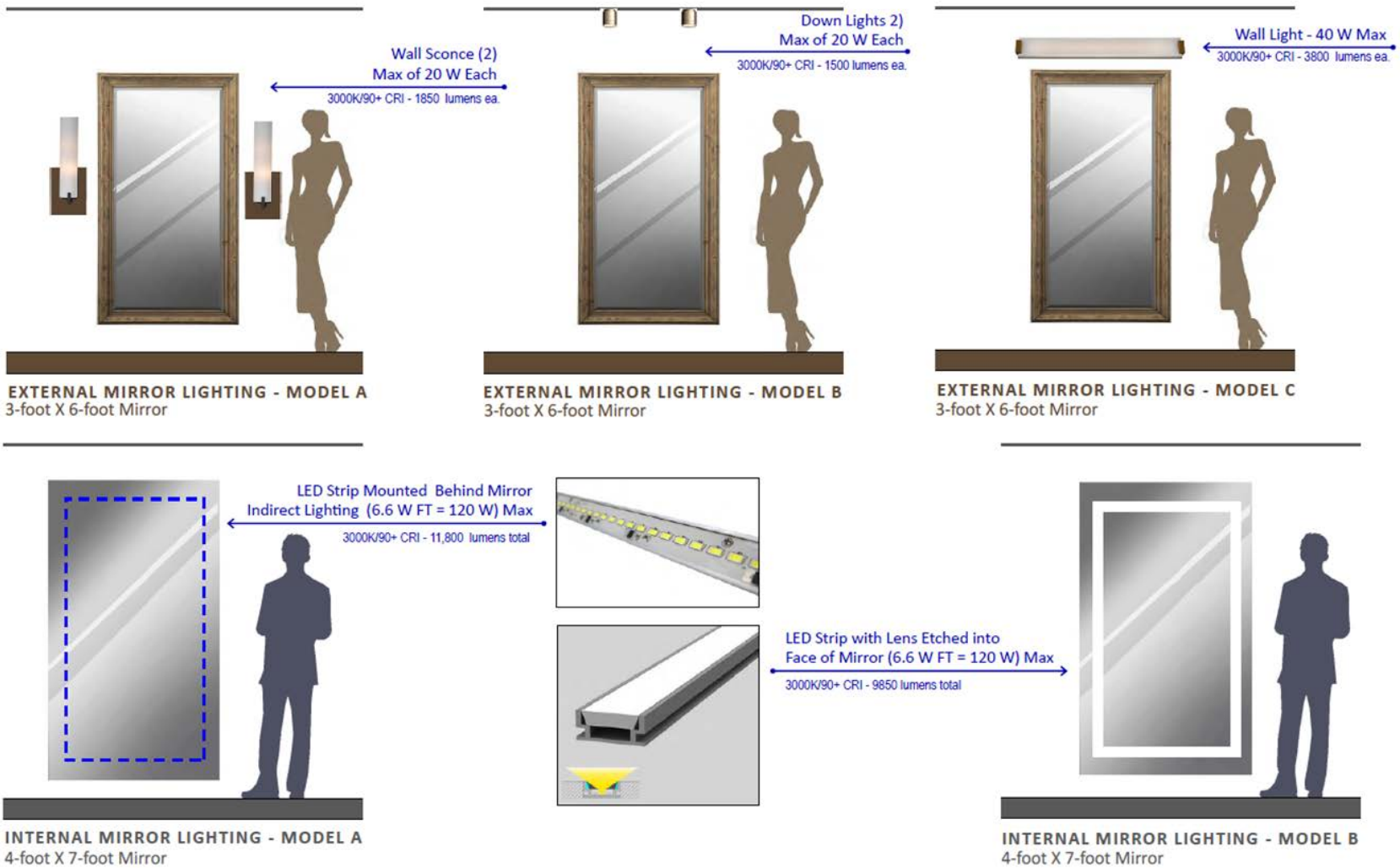
Figure 38: Models used for developing mirror lighting wattage allowance in Area Category Method.
