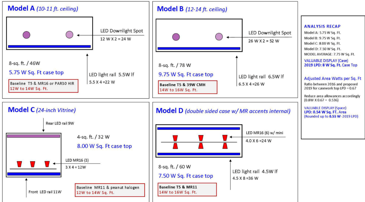
Figure 29: Model study for valuable display allowance. 11
