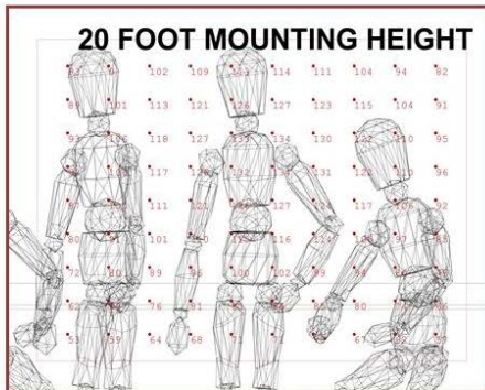
Figure 27: AGi32 Model study for accent/display case lighting applications.
