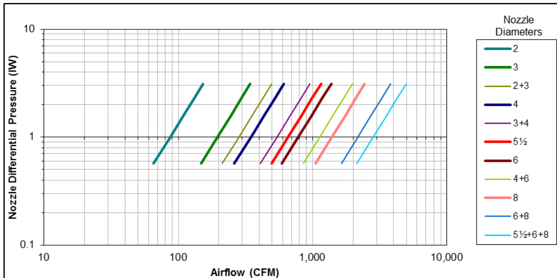
Figure 18: Airflow apparatus operating range
