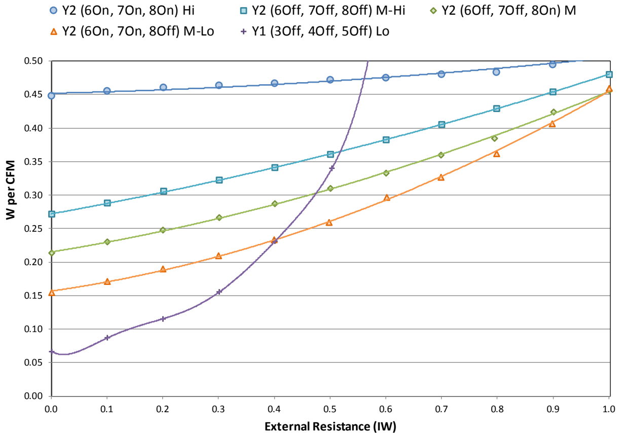
Figure 15: Fan efficacy test results – Carrier 59TP6A060E171214
