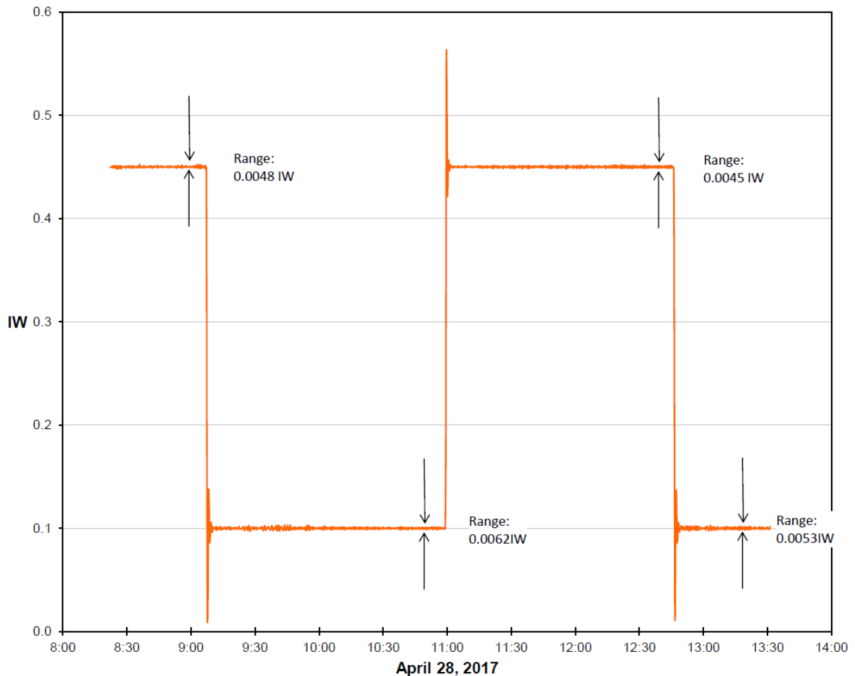
Figure 20: Recent test holding fixed backpressure
