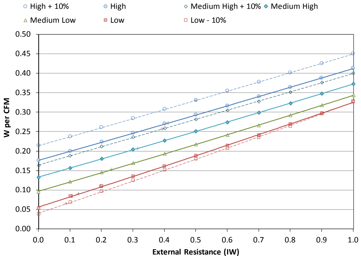
Figure 14: Typical fan efficacy test results – Lennox SL280UH090XV48B
