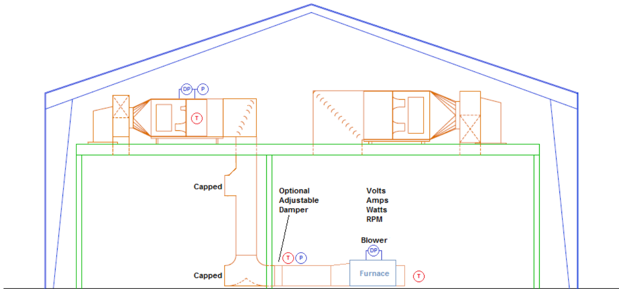
Figure 17: HVAC lab setup for furnace tests
