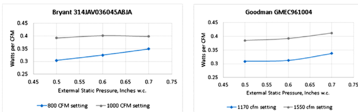
Figure 13: Preliminary lab test results for two ECM furnaces
