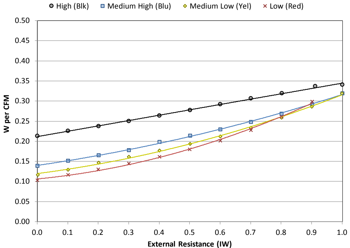
Figure 16: Fan efficacy results – Trane XT95 TDH1B04A9H21BA
