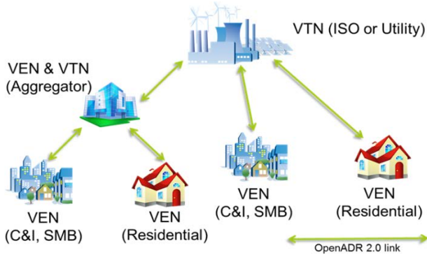
Figure 6: Configuration of communication using OpenADR 2.0 links from signaller to on-Site VEN
