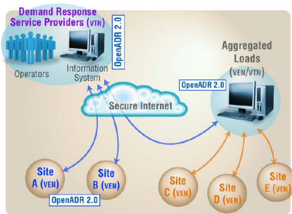
Figure 7: Configuration of communication using OpenADR 2.0 links from signaller to off-site VEN to site
