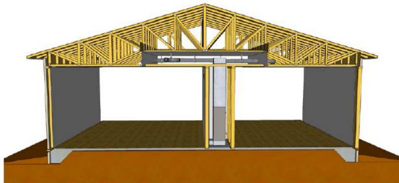
Figure 6: Interior Furnace with Ducts in Conditioned Plenum Space (IBACOS 2013)
