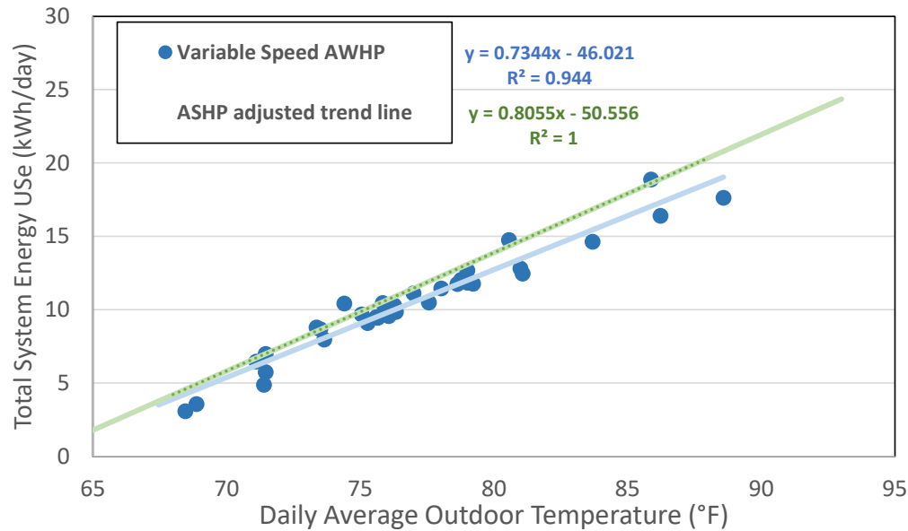
Figure 6: Comparison of monitored variable speed AWHP and model adjusted prescriptive ASHP cooling energy use as a function of daily average outdoor air temperature
