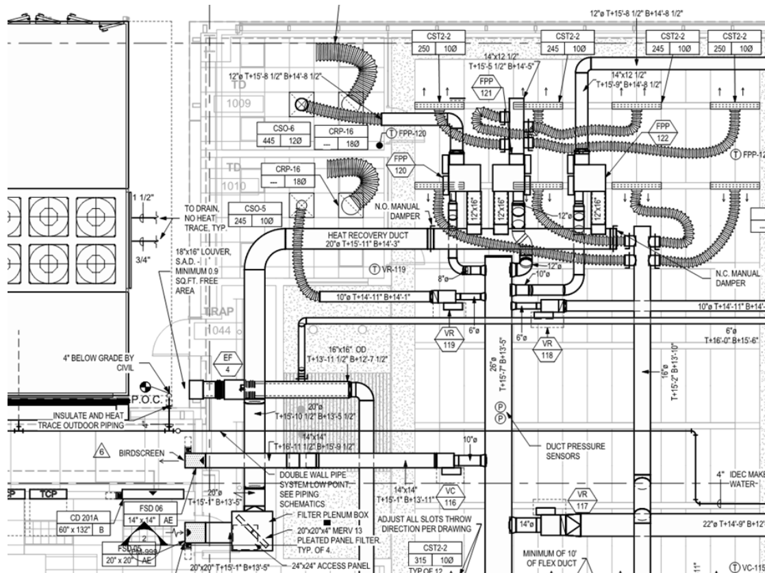
Figure 2. Computer room heat recovery example mechanical plan: fan powered boxes.
