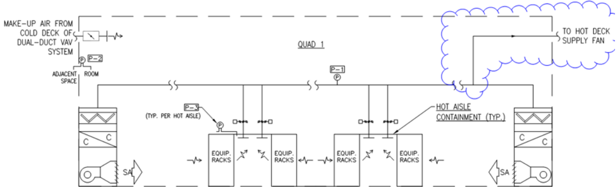
Figure 1. Computer room heat recovery example mechanical diagram: DFDD.
