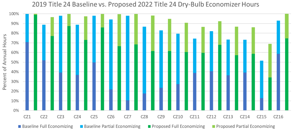
Figure 5. Comparison of 2019 Title 24 and proposed 2022 Title 24 dry-bulb economizing hours.
