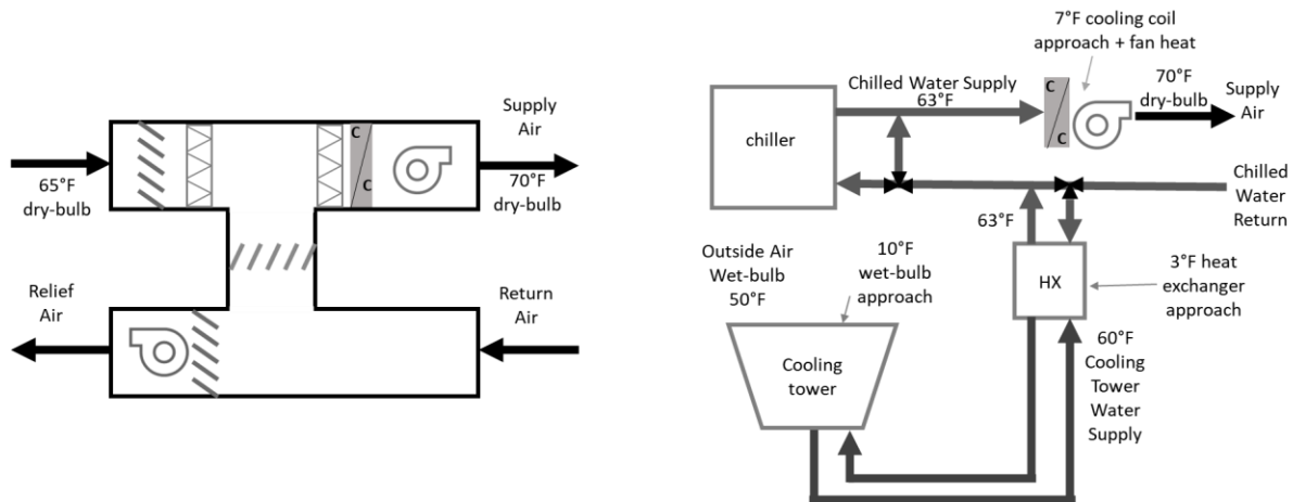
Figure 4. Example design temperatures: air economizer (left) and water economizer (right).
