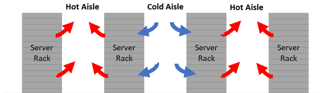
Figure 3. Hot aisle/cold aisle server arrangement schematic.
