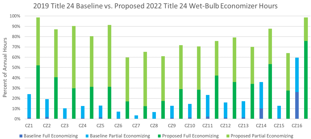
Figure 6. Comparison of 2019 Title 24 and proposed 2022 Title 24 wet-bulb economizing hours.
