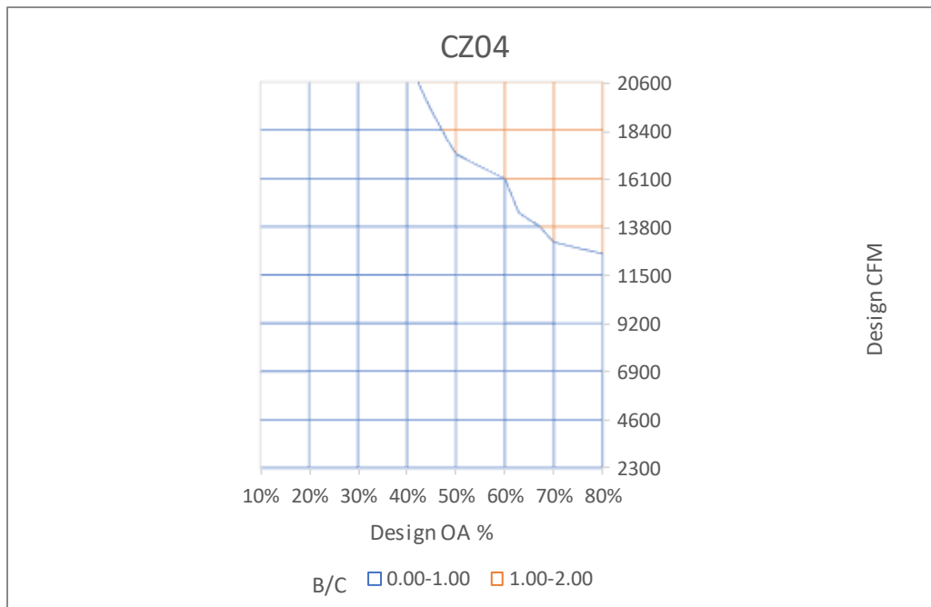
Figure 43: Cost effectiveness of EAHR in CZ4 with 4,644 hours of operation.
