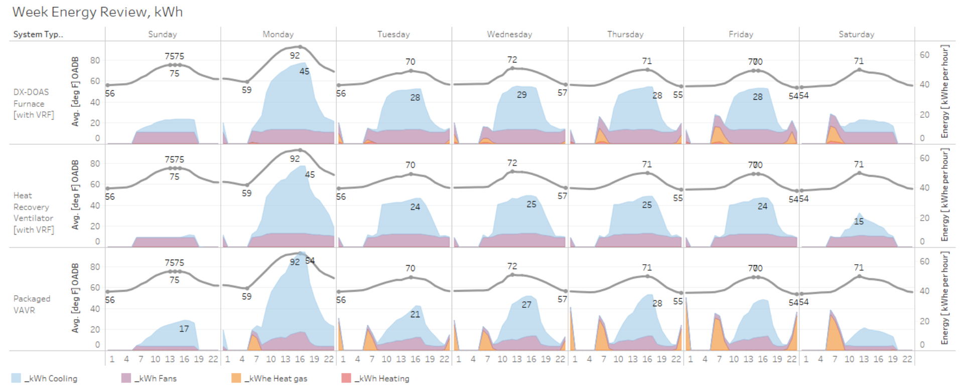
Figure 31: HVAC-only load profile comparison for systems in Climate Zone 4, Week 37 (Medium Offices)
