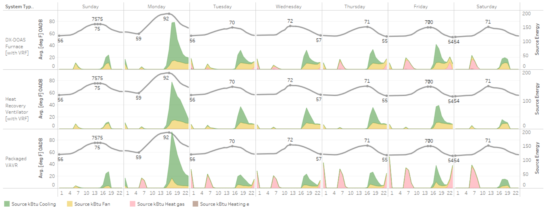
Figure 33: Source energy load profile comparison for systems in Climate Zone 4, Week 37 (Medium Offices)
