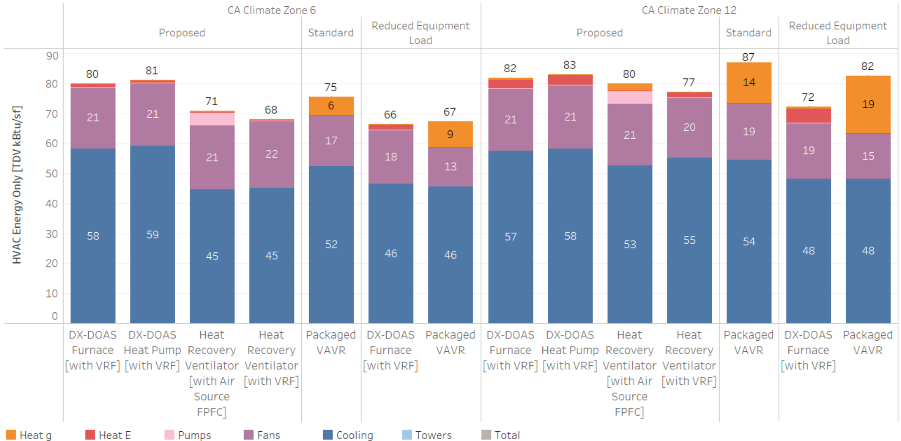
Figure 27: System comparison of HVAC-only TDV site energy for Climate Zone 6 and Climate Zone 12 for Medium Office.
