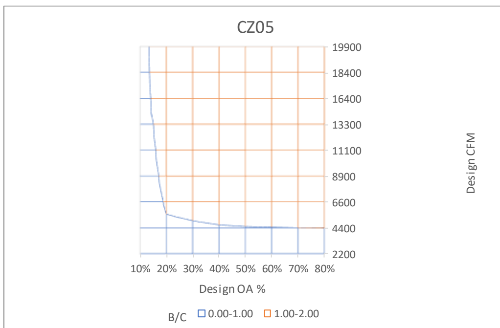
Figure 56: Cost effectiveness of EAHR in CZ 5 with 8,760 hours of operation.
