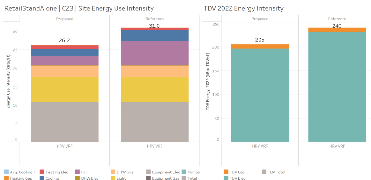
Figure 9: TDV energy and site energy results, Retail Stand Alone, Climate Zone 3.
