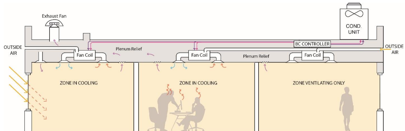
Figure 1: Small nonresidential HVAC system with directly ducted outdoor air to fan coils.
