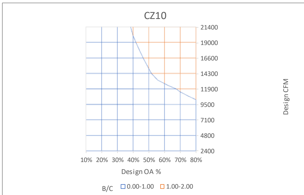
Figure 45: Cost effectiveness of EAHR in CZ10 with 4,644 hours of operation.
