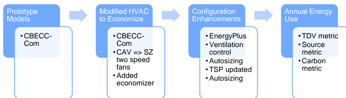
Figure 23: Diagram illustrating work-flow mixed-air systems
