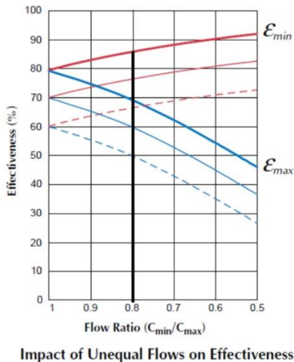
Figure 21: Effectiveness to flow ratio of supply and return, ASHRAE.
