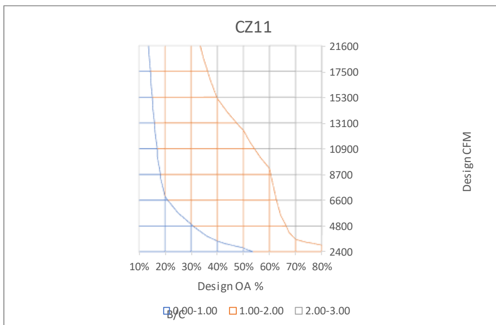
Figure 46: Cost effectiveness of EAHR in CZ11 with 4,644 hours of operation.
