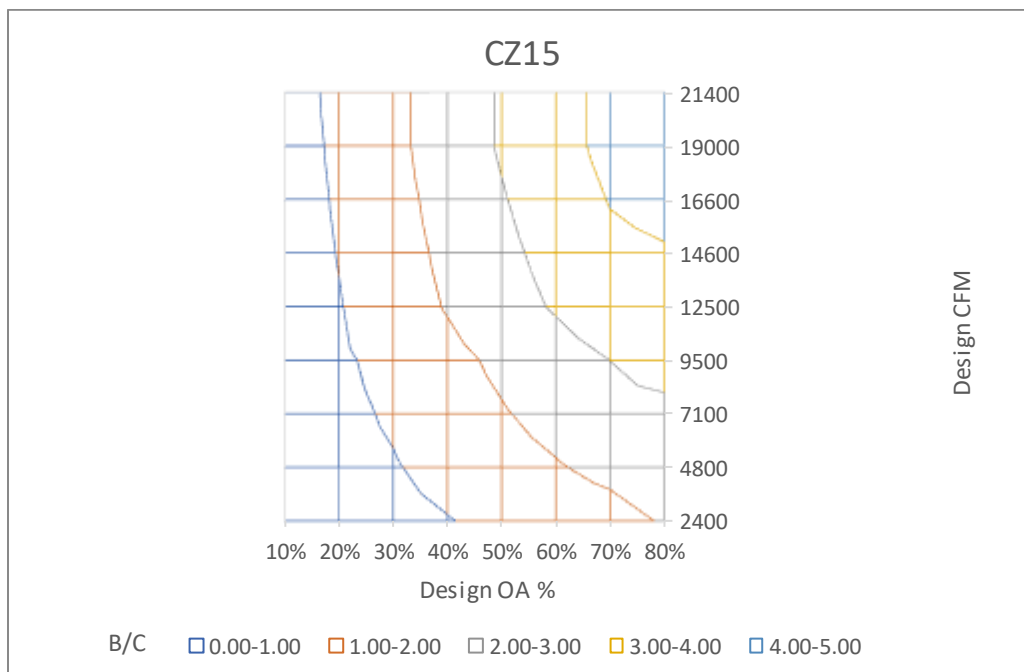
Figure 50: Cost effectiveness of EAHR in CZ15 with 4,644 hours of operation.
