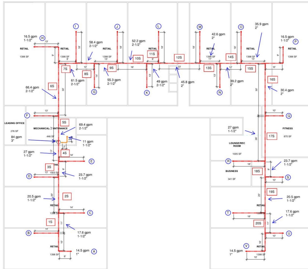
Figure 15 - Mid-Rise Mixed-Use Proposed Distribution Piping
