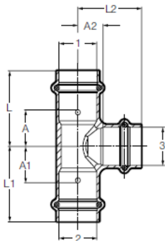
Figure 22: Example of a tee fitting.
