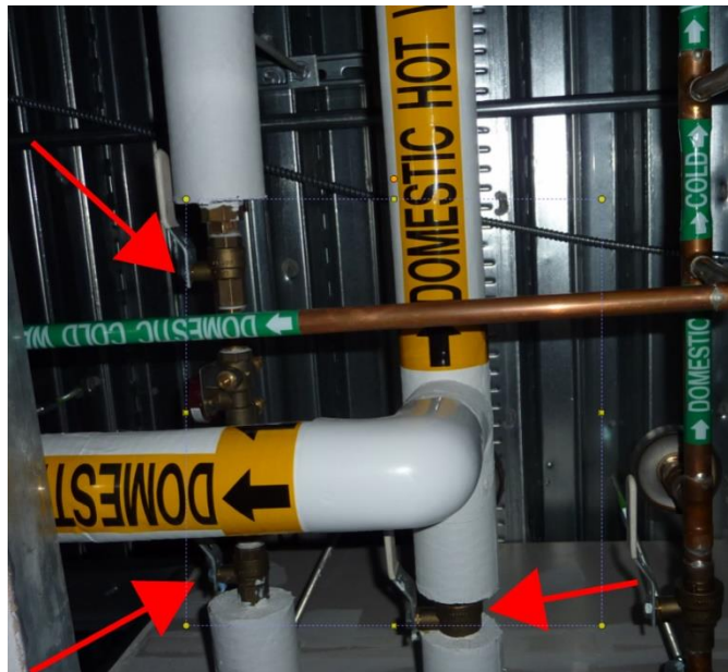
Figure 9: Uninsulated valves.
