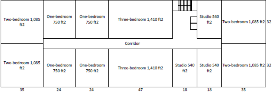
Figure 37: Low-rise loaded corridor second and third floor plan.
