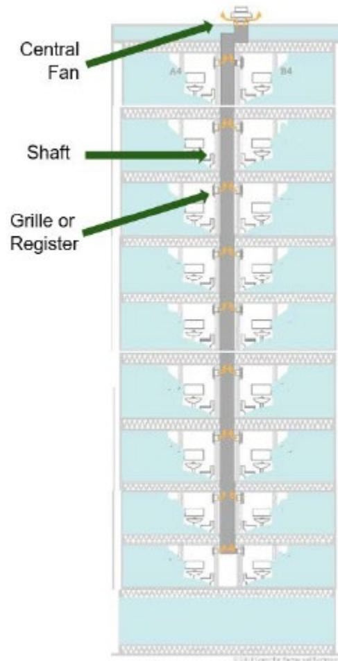
Figure 1. Diagram of central ventilation system (Center for Energy and Environment 2016)
