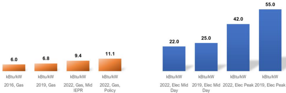
Figure 24: Comparison of TDV costs from 2019 and 2022 for Climate Zone 12
