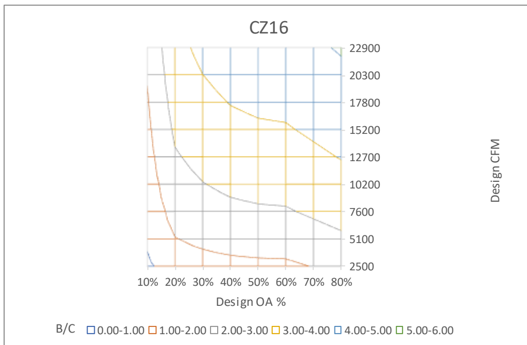
Figure 65: Cost effectiveness of EAHR in CZ 16 with 8,760 hours of operation.
