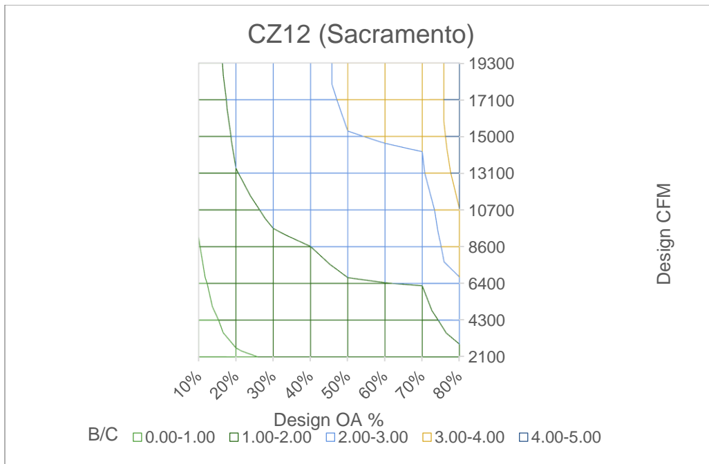
Figure 61: Cost effectiveness of EAHR in CZ 12 with 8,760 hours of operation.
