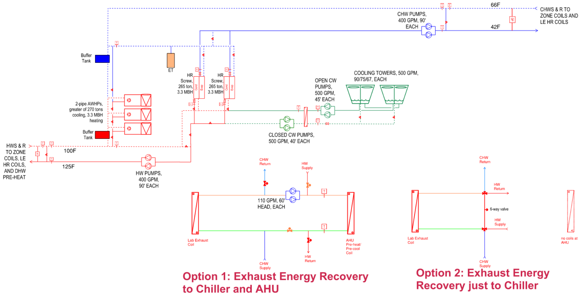
Figure 5. Schematic of lab exhaust to heat recovery chiller.
