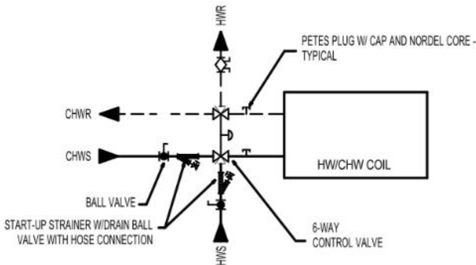
Figure 19: 6-Way changeover valve piping schematic.
