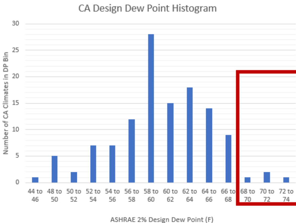
Figure 15: California design dew point histogram.
