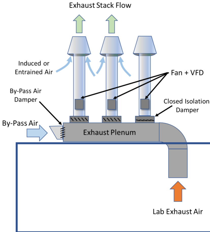
Figure 6: Components of lab exhaust flows.
