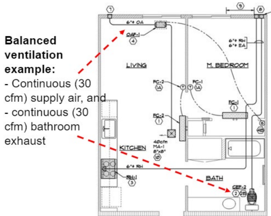
Figure 8: Example of balanced ventilation without heat recovery
