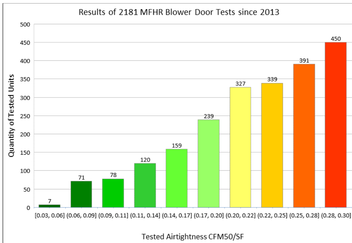
Figure 11: Results of over 2,000 U.S. multifamily dwelling unit blower door tests from 2013 to 2019
