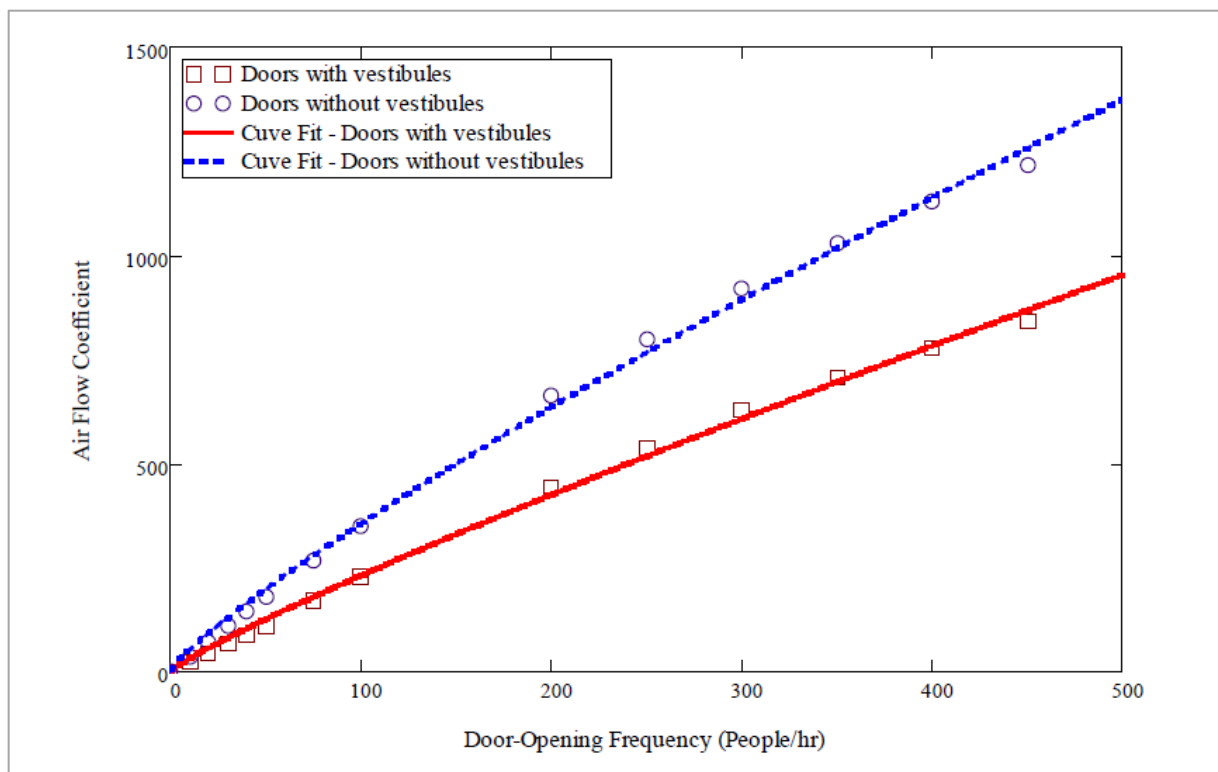
Figure 2: Air flow coefficient vs door opening frequency
